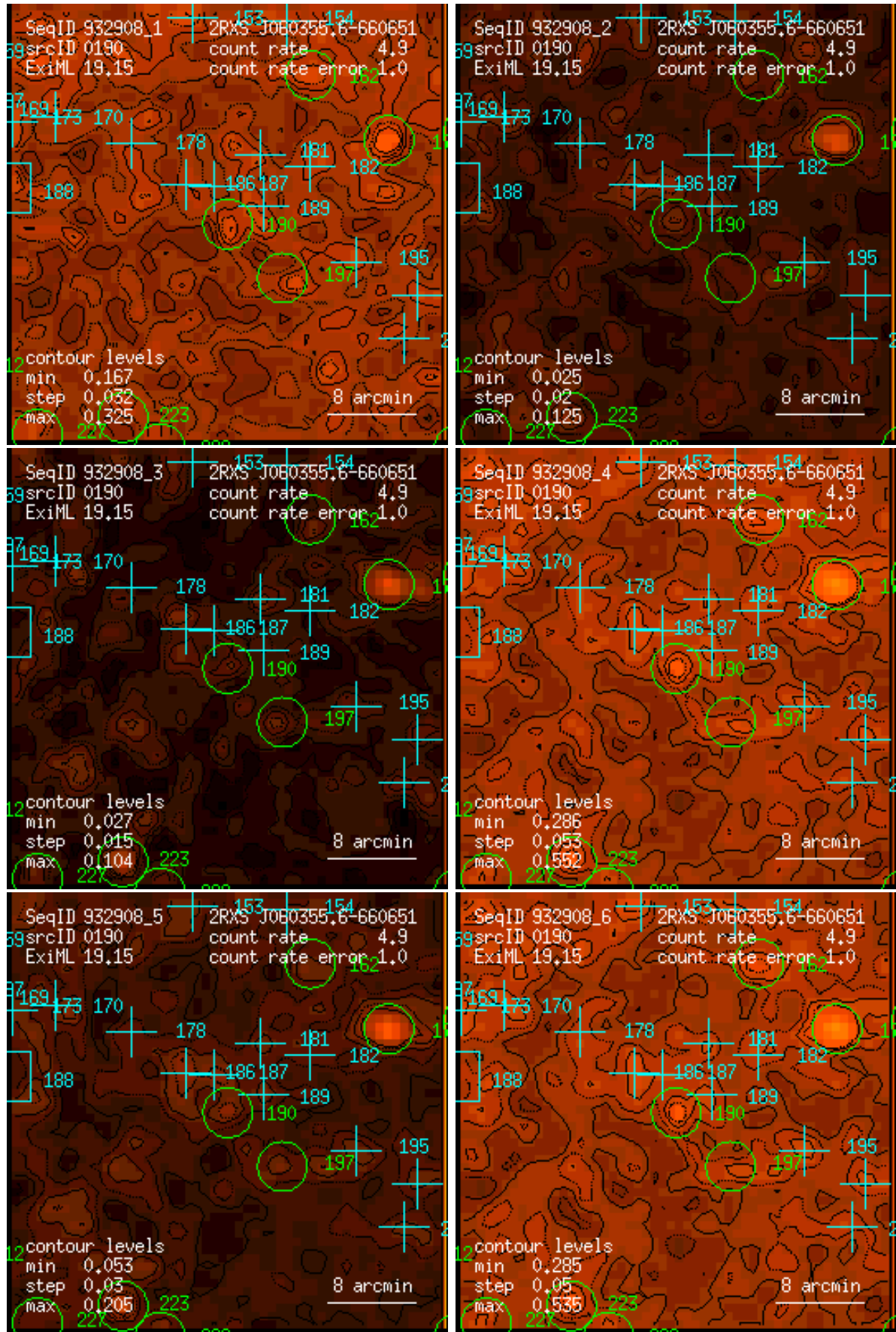
Figure 190: RASS 932908: detection 0190: band rate images, Gaussian filter: (1) PSPC channels 11 – 41, (2) 52 – 90, (3) 91 – 201, (4) 11 – 235, (5) 52 – 201, (6) 11 – 201. Broad band rates in counts/ks. Band rate contour levels in counts/ks/arcmin 2 .
