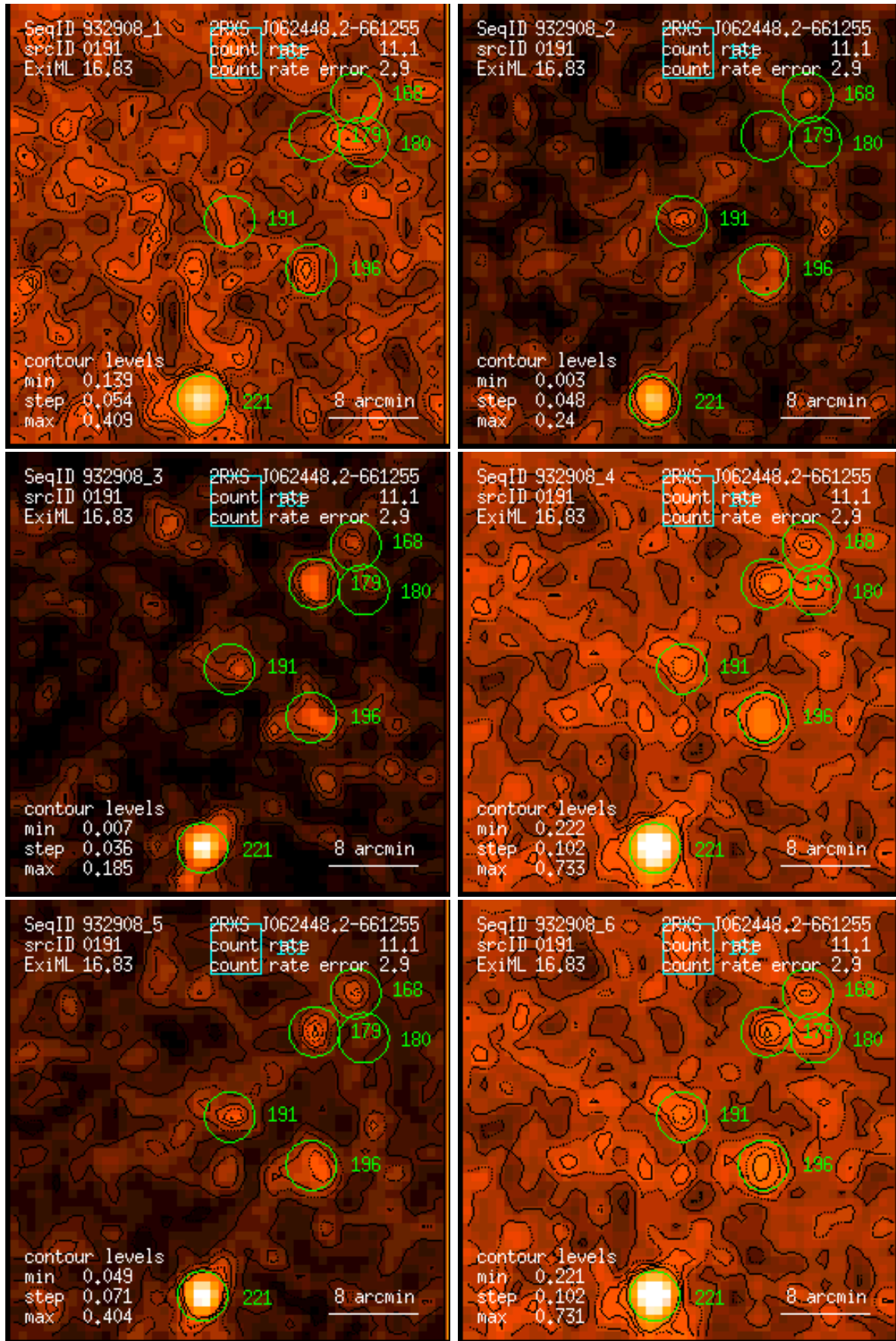
Figure 191: RASS 932908: detection 0191: band rate images, Gaussian filter: (1) PSPC channels 11 – 41, (2) 52 – 90, (3) 91 – 201, (4) 11 – 235, (5) 52 – 201, (6) 11 – 201. Broad band rates in counts/ks. Band rate contour levels in counts/ks/arcmin 2 .
