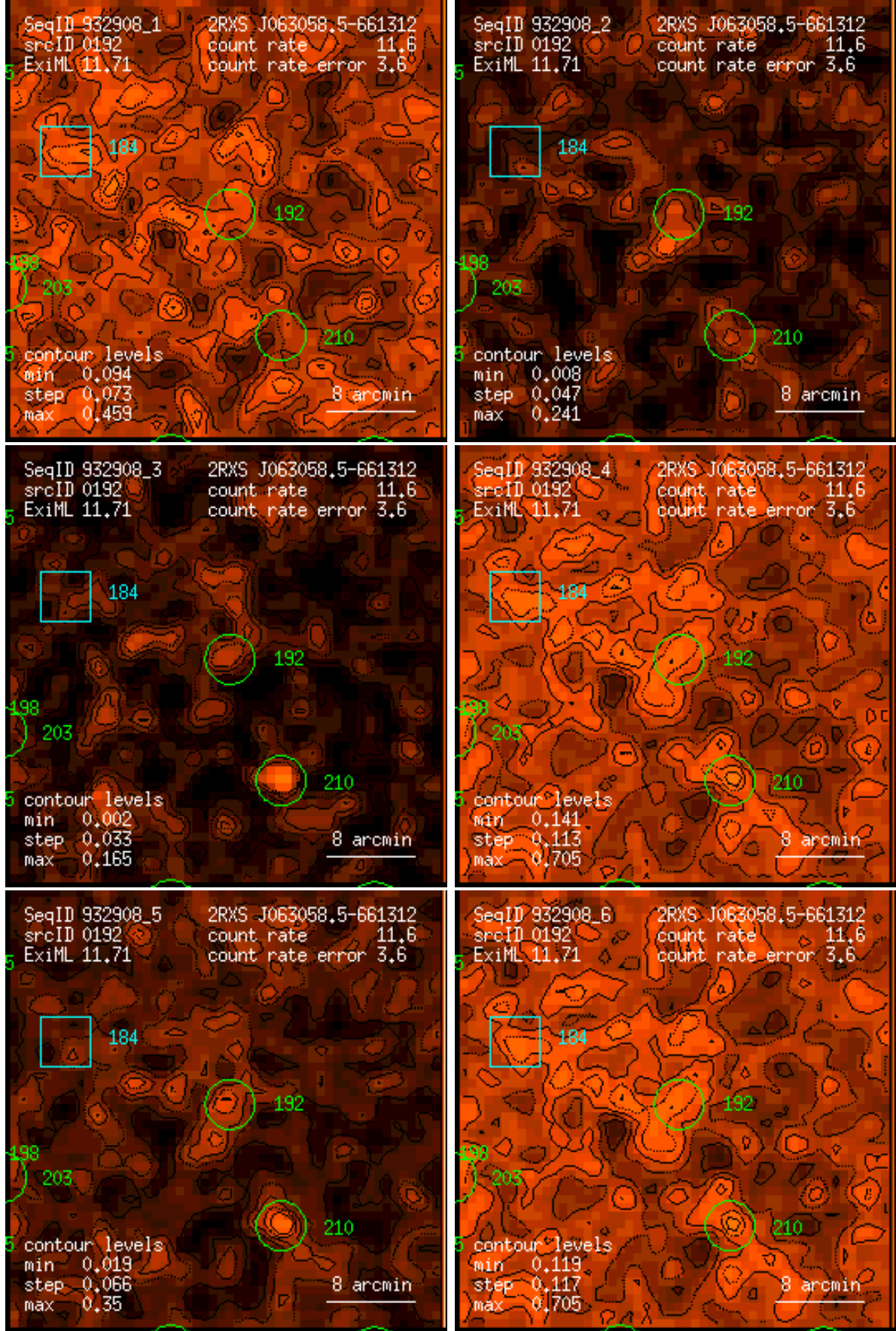
Figure 192: RASS 932908: detection 0192: band rate images, Gaussian filter: (1) PSPC channels 11 – 41, (2) 52 – 90, (3) 91 – 201, (4) 11 – 235, (5) 52 – 201, (6) 11 – 201. Broad band rates in counts/ks. Band rate contour levels in counts/ks/arcmin 2 .
