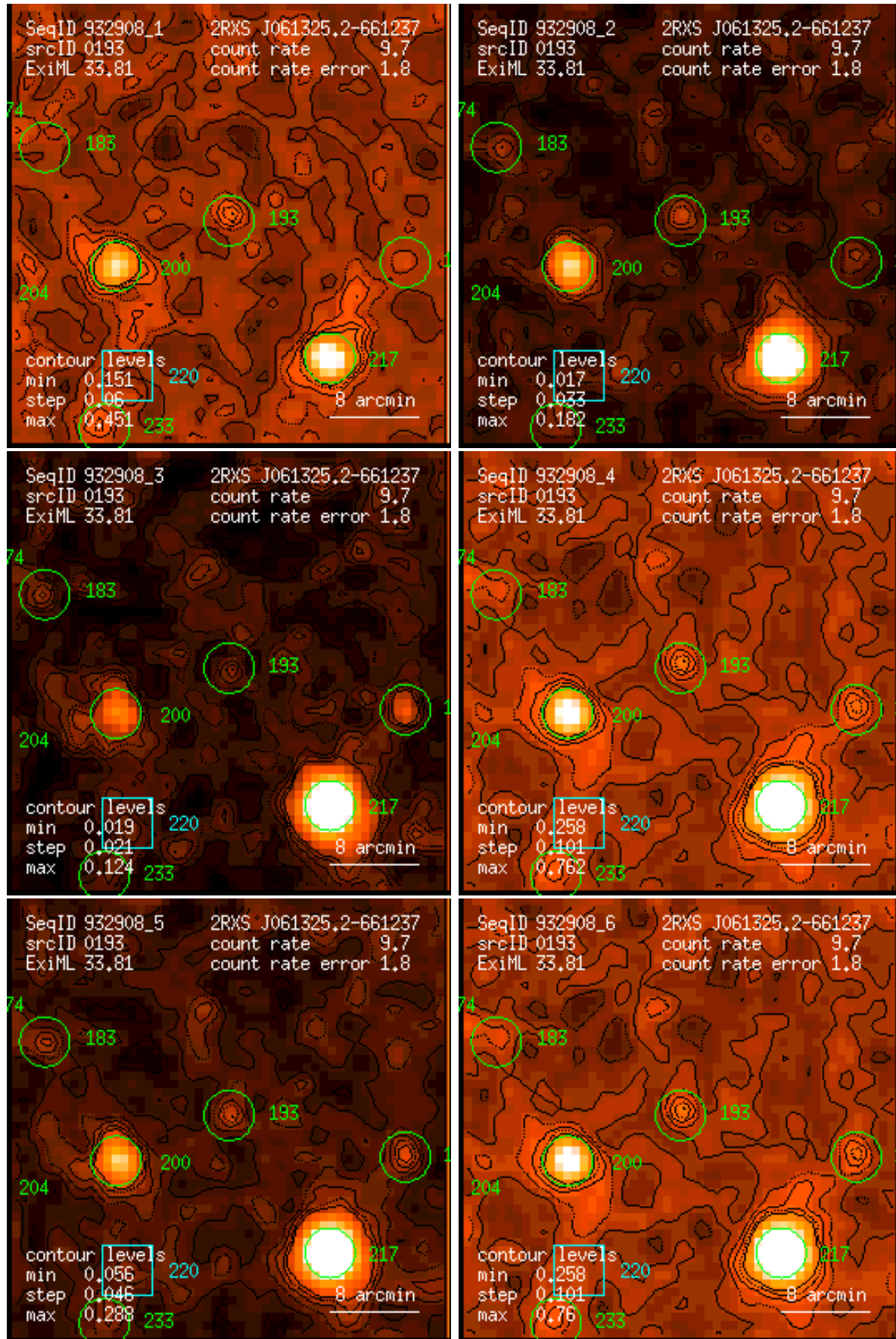
Figure 193: RASS 932908: detection 0193: band rate images, Gaussian filter: (1) PSPC channels 11 – 41, (2) 52 – 90, (3) 91 – 201, (4) 11 – 235, (5) 52 – 201, (6) 11 – 201. Broad band rates in counts/ks. Band rate contour levels in counts/ks/arcmin 2 .
