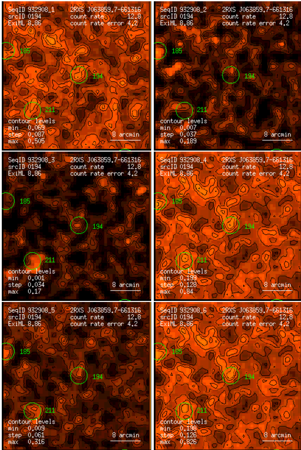
Figure 194: RASS 932908: detection 0194: band rate images, Gaussian filter: (1) PSPC channels 11 – 41, (2) 52 – 90, (3) 91 – 201, (4) 11 – 235, (5) 52 – 201, (6) 11 – 201. Broad band rates in counts/ks. Band rate contour levels in counts/ks/arcmin 2 .
