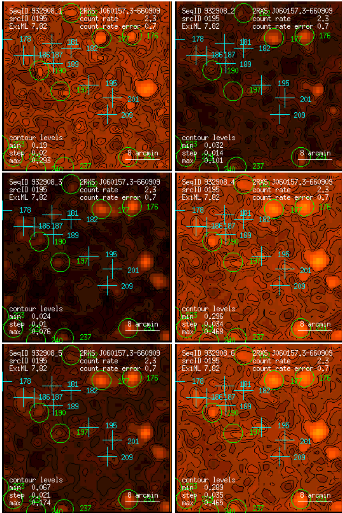
Figure 195: RASS 932908: detection 0195: band rate images, Gaussian filter: (1) PSPC channels 11 – 41, (2) 52 – 90, (3) 91 – 201, (4) 11 – 235, (5) 52 – 201, (6) 11 – 201. Broad band rates in counts/ks. Band rate contour levels in counts/ks/arcmin 2 .
