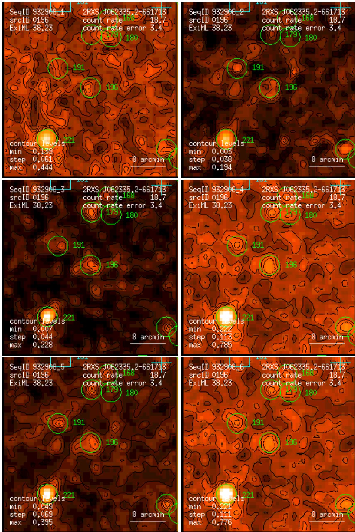
Figure 196: RASS 932908: detection 0196: band rate images, Gaussian filter: (1) PSPC channels 11 – 41, (2) 52 – 90, (3) 91 – 201, (4) 11 – 235, (5) 52 – 201, (6) 11 – 201. Broad band rates in counts/ks. Band rate contour levels in counts/ks/arcmin 2 .
