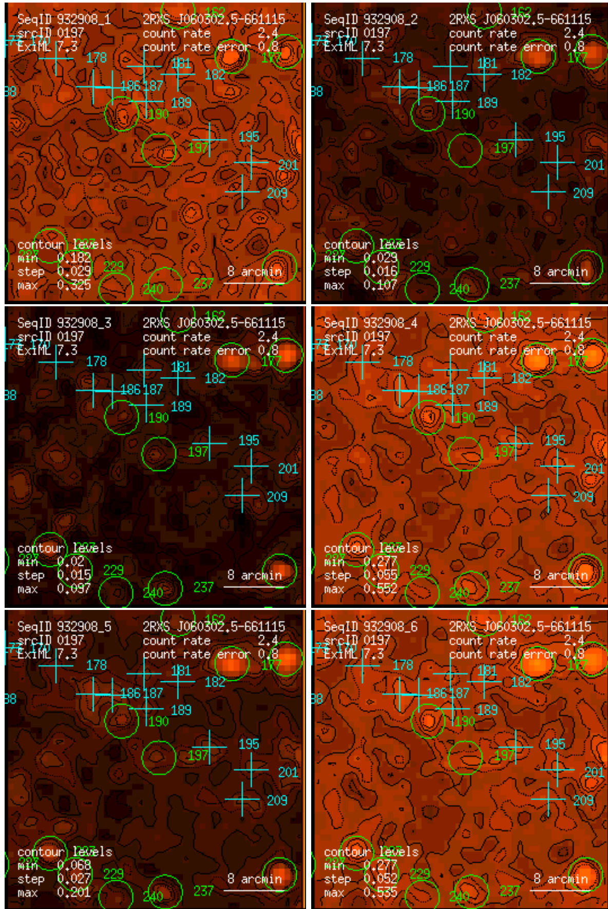
Figure 197: RASS 932908: detection 0197: band rate images, Gaussian filter: (1) PSPC channels 11 – 41, (2) 52 – 90, (3) 91 – 201, (4) 11 – 235, (5) 52 – 201, (6) 11 – 201. Broad band rates in counts/ks. Band rate contour levels in counts/ks/arcmin 2 .
