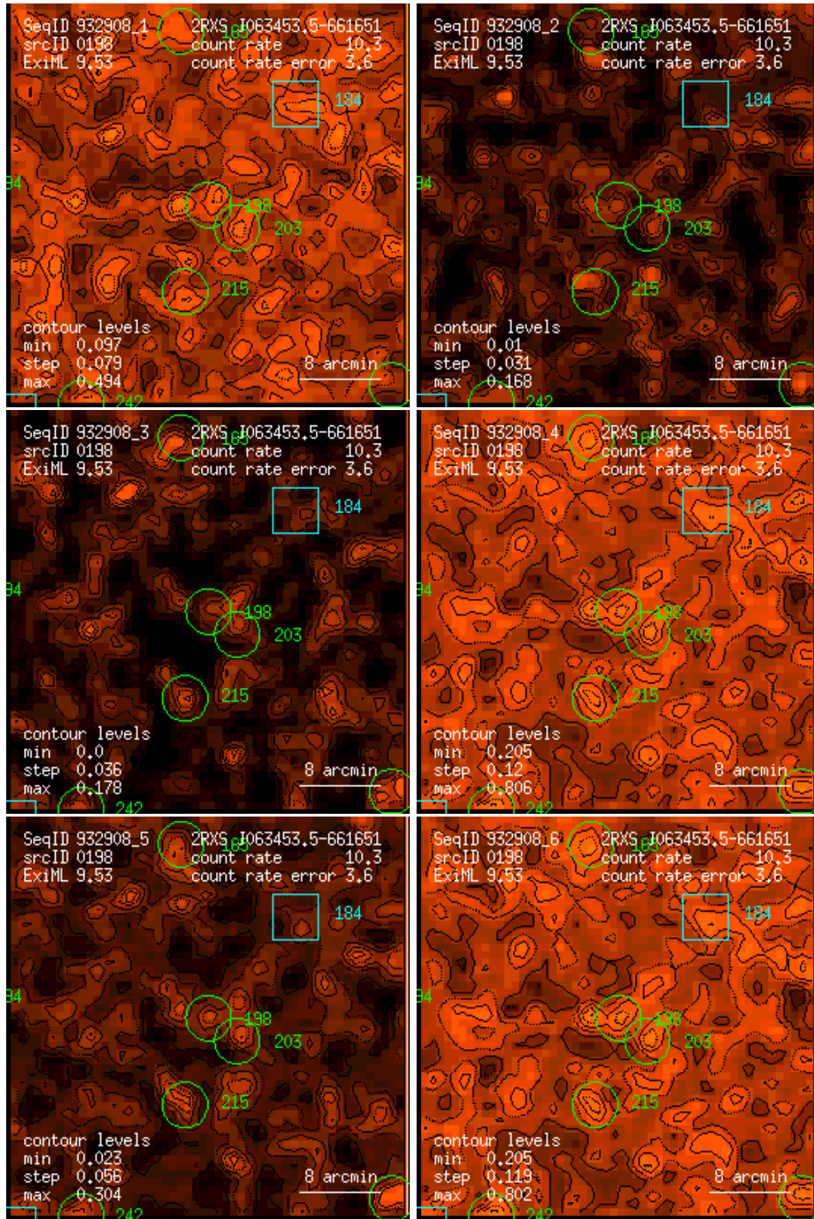
Figure 198: RASS 932908: detection 0198: band rate images, Gaussian filter: (1) PSPC channels 11 – 41, (2) 52 – 90, (3) 91 – 201, (4) 11 – 235, (5) 52 – 201, (6) 11 – 201. Broad band rates in counts/ks. Band rate contour levels in counts/ks/arcmin 2 .
