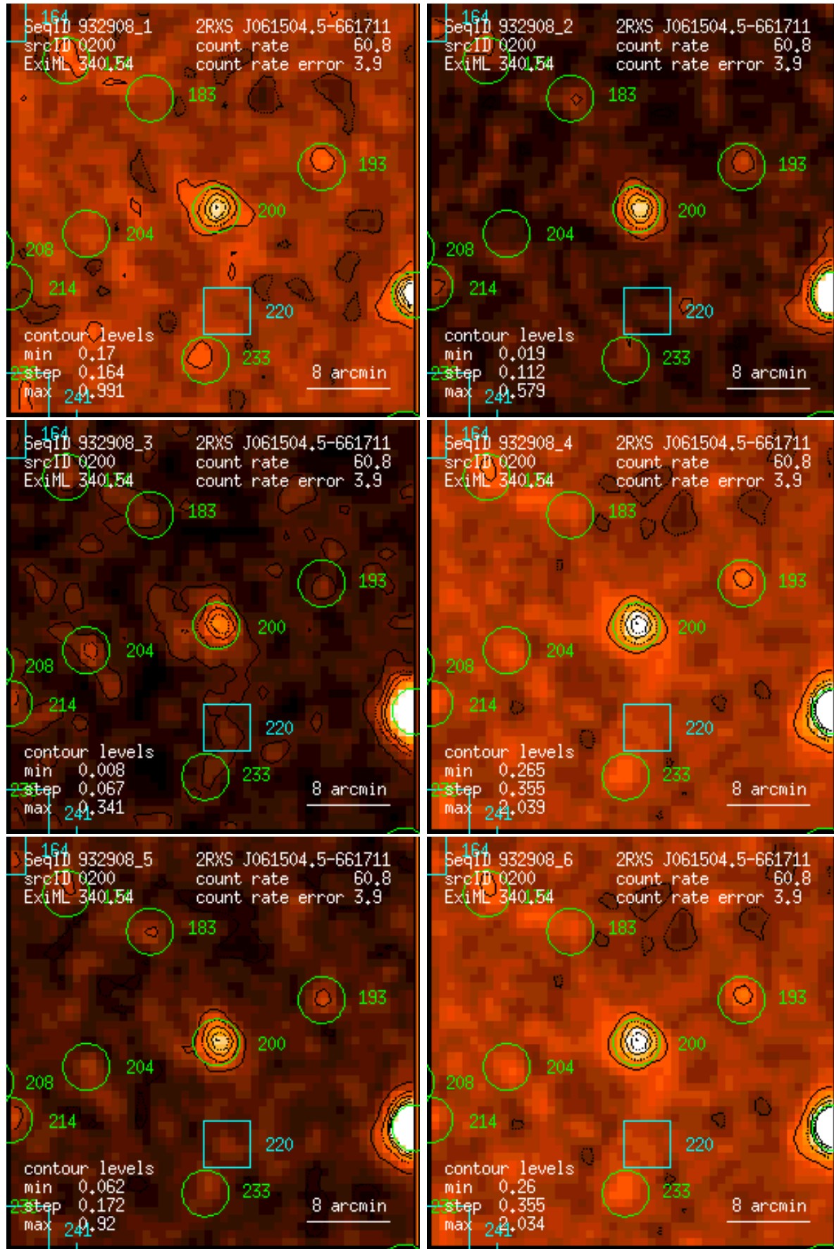
Figure 200: RASS 932908: detection 0200: band rate images, Gaussian filter: (1) PSPC channels 11 – 41, (2) 52 – 90, (3) 91 – 201, (4) 11 – 235, (5) 52 – 201, (6) 11 – 201. Broad band rates in counts/ks. Band rate contour levels in counts/ks/arcmin 2 .
