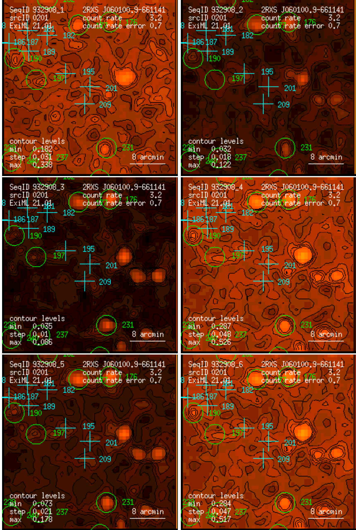
Figure 201: RASS 932908: detection 0201: band rate images, Gaussian filter: (1) PSPC channels 11 – 41, (2) 52 – 90, (3) 91 – 201, (4) 11 – 235, (5) 52 – 201, (6) 11 – 201. Broad band rates in counts/ks. Band rate contour levels in counts/ks/arcmin 2 .
