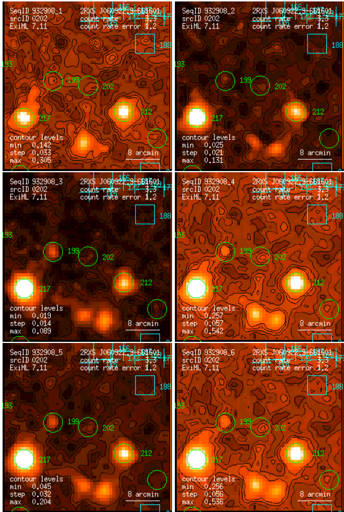
Figure 202: RASS 932908: detection 0202: band rate images, Gaussian filter: (1) PSPC channels 11 – 41, (2) 52 – 90, (3) 91 – 201, (4) 11 – 235, (5) 52 – 201, (6) 11 – 201. Broad band rates in counts/ks. Band rate contour levels in counts/ks/arcmin 2 .
