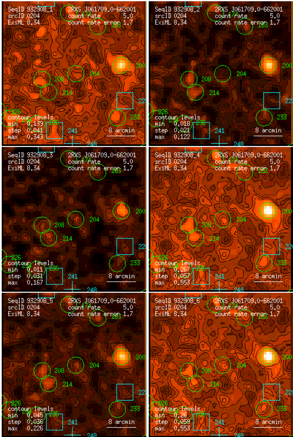
Figure 204: RASS 932908: detection 0204: band rate images, Gaussian filter: (1) PSPC channels 11 – 41, (2) 52 – 90, (3) 91 – 201, (4) 11 – 235, (5) 52 – 201, (6) 11 – 201. Broad band rates in counts/ks. Band rate contour levels in counts/ks/arcmin 2 .
