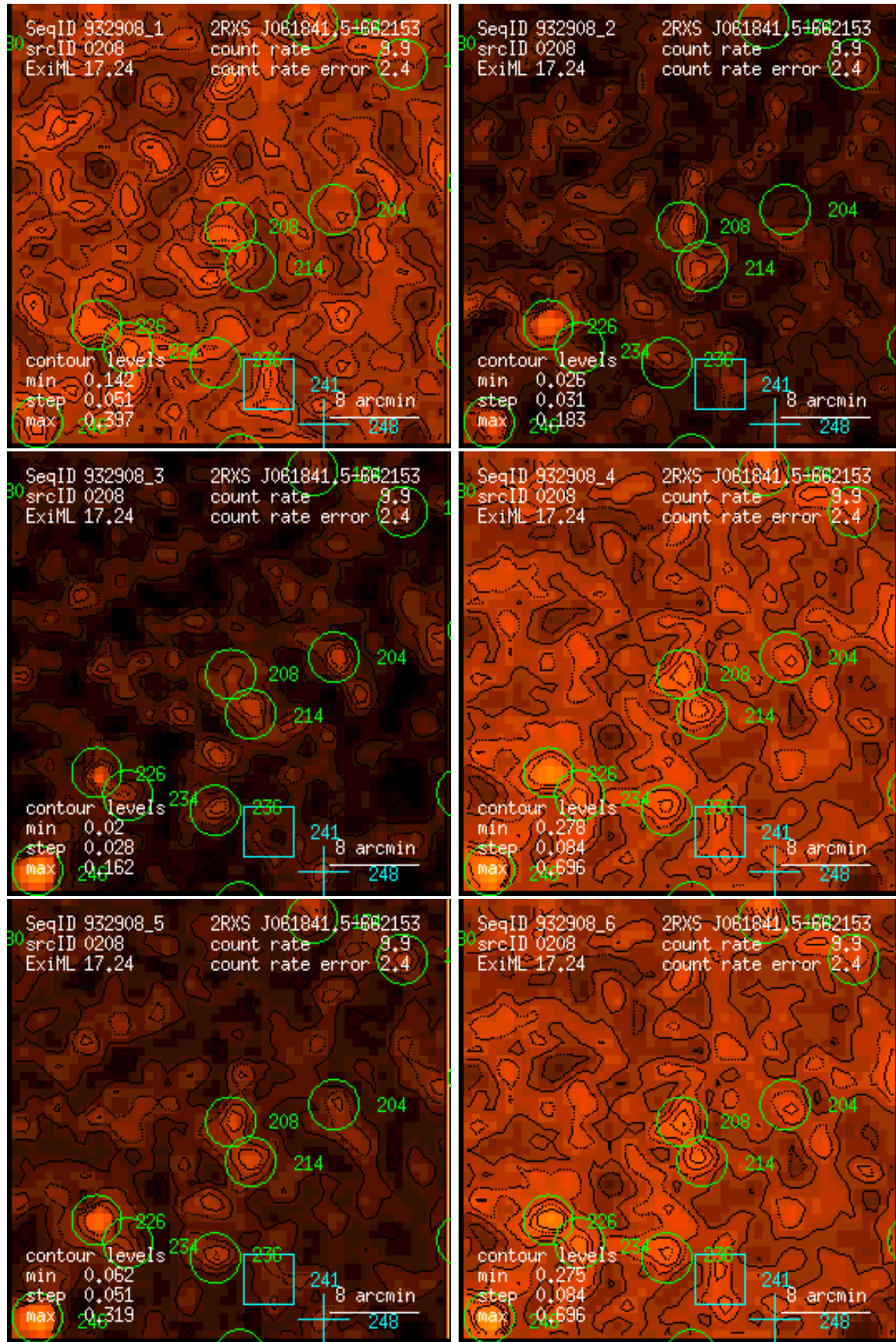
Figure 208: RASS 932908: detection 0208: band rate images, Gaussian filter: (1) PSPC channels 11 – 41, (2) 52 – 90, (3) 91 – 201, (4) 11 – 235, (5) 52 – 201, (6) 11 – 201. Broad band rates in counts/ks. Band rate contour levels in counts/ks/arcmin 2 .
