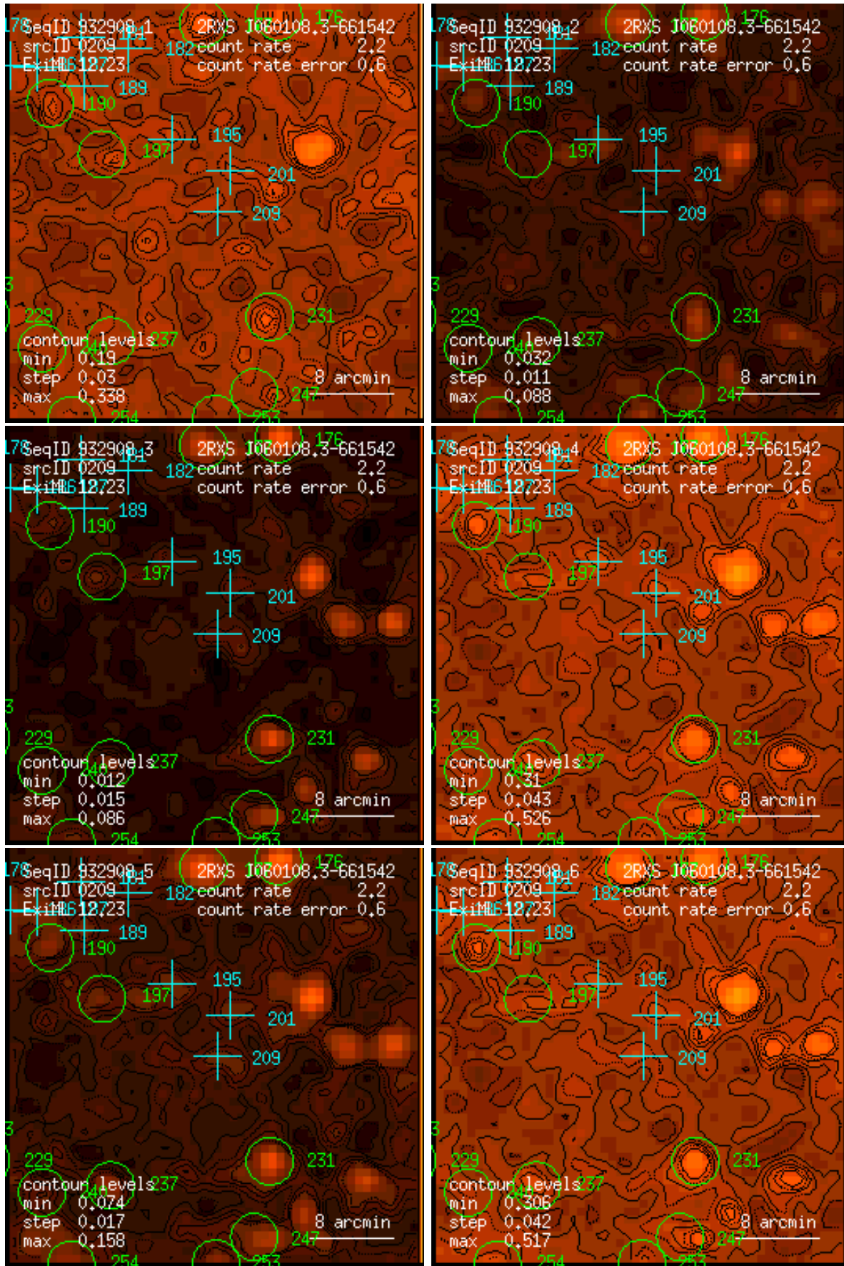
Figure 209: RASS 932908: detection 0209: band rate images, Gaussian filter: (1) PSPC channels 11 – 41, (2) 52 – 90, (3) 91 – 201, (4) 11 – 235, (5) 52 – 201, (6) 11 – 201. Broad band rates in counts/ks. Band rate contour levels in counts/ks/arcmin 2 .
