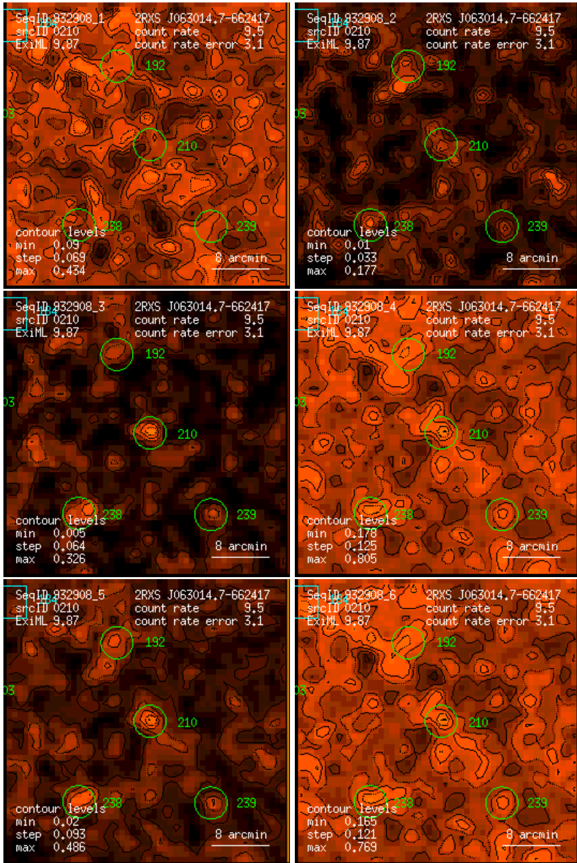
Figure 210: RASS 932908: detection 0210: band rate images, Gaussian filter: (1) PSPC channels 11 – 41, (2) 52 – 90, (3) 91 – 201, (4) 11 – 235, (5) 52 – 201, (6) 11 – 201. Broad band rates in counts/ks. Band rate contour levels in counts/ks/arcmin 2 .
