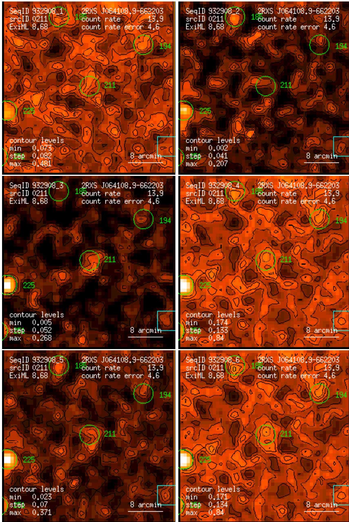
Figure 211: RASS 932908: detection 0211: band rate images, Gaussian filter: (1) PSPC channels 11 – 41, (2) 52 – 90, (3) 91 – 201, (4) 11 – 235, (5) 52 – 201, (6) 11 – 201. Broad band rates in counts/ks. Band rate contour levels in counts/ks/arcmin 2 .
