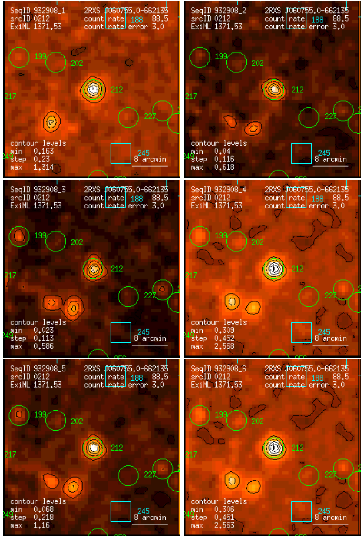
Figure 212: RASS 932908: detection 0212: band rate images, Gaussian filter: (1) PSPC channels 11 – 41, (2) 52 – 90, (3) 91 – 201, (4) 11 – 235, (5) 52 – 201, (6) 11 – 201. Broad band rates in counts/ks. Band rate contour levels in counts/ks/arcmin 2 .
