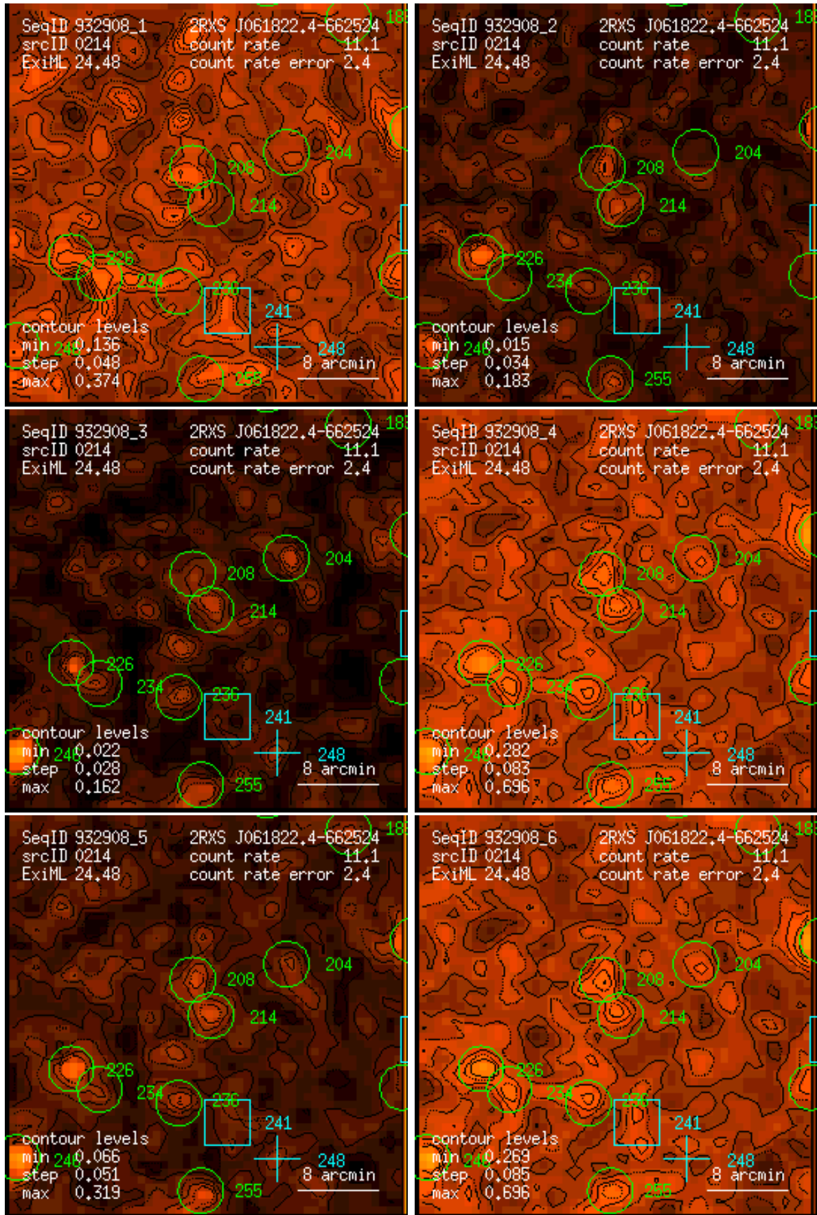
Figure 214: RASS 932908: detection 0214: band rate images, Gaussian filter: (1) PSPC channels 11 – 41, (2) 52 – 90, (3) 91 – 201, (4) 11 – 235, (5) 52 – 201, (6) 11 – 201. Broad band rates in counts/ks. Band rate contour levels in counts/ks/arcmin 2 .
