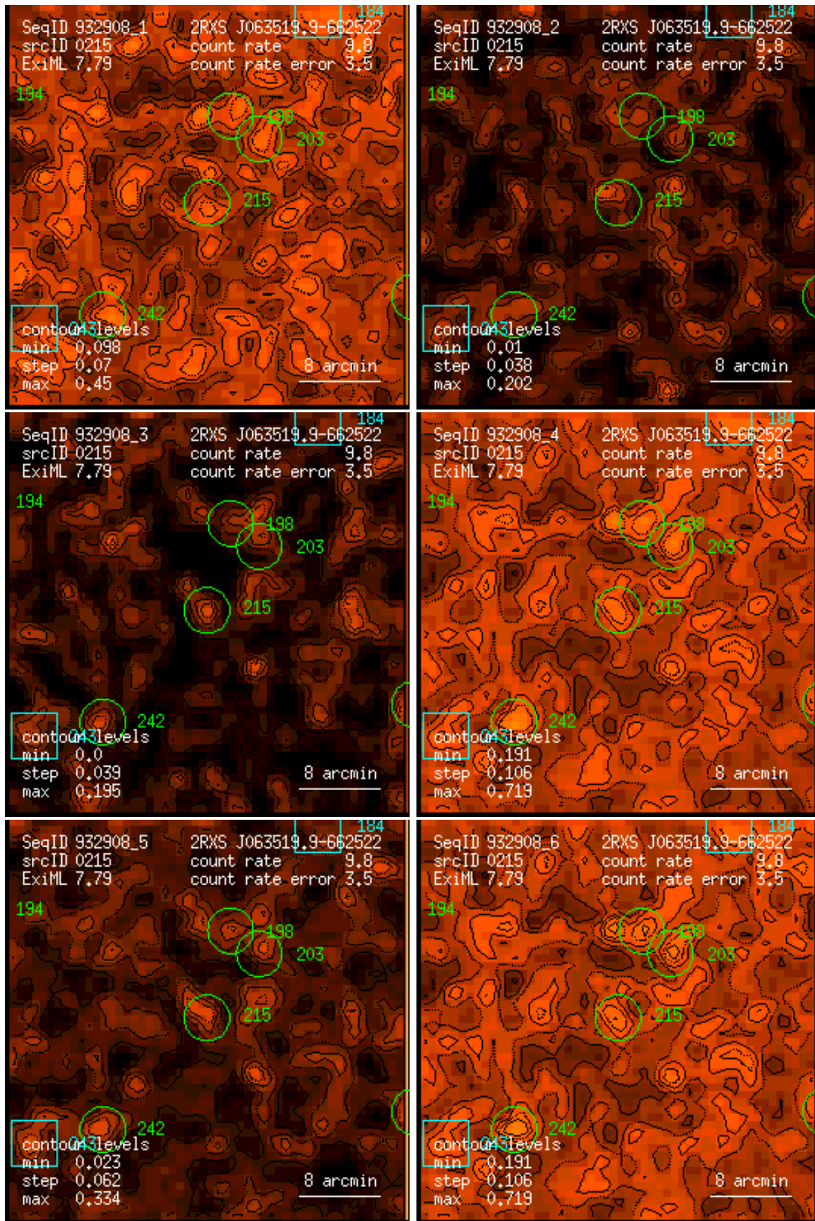
Figure 215: RASS 932908: detection 0215: band rate images, Gaussian filter: (1) PSPC channels 11 – 41, (2) 52 – 90, (3) 91 – 201, (4) 11 – 235, (5) 52 – 201, (6) 11 – 201. Broad band rates in counts/ks. Band rate contour levels in counts/ks/arcmin 2 .
