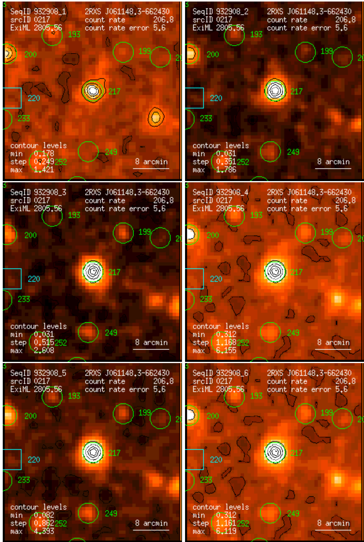
Figure 217: RASS 932908: detection 0217: band rate images, Gaussian filter: (1) PSPC channels 11 – 41, (2) 52 – 90, (3) 91 – 201, (4) 11 – 235, (5) 52 – 201, (6) 11 – 201. Broad band rates in counts/ks. Band rate contour levels in counts/ks/arcmin 2 .
