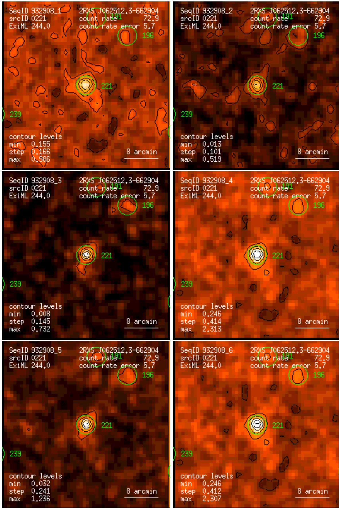
Figure 221: RASS 932908: detection 0221: band rate images, Gaussian filter: (1) PSPC channels 11 – 41, (2) 52 – 90, (3) 91 – 201, (4) 11 – 235, (5) 52 – 201, (6) 11 – 201. Broad band rates in counts/ks. Band rate contour levels in counts/ks/arcmin 2 .
