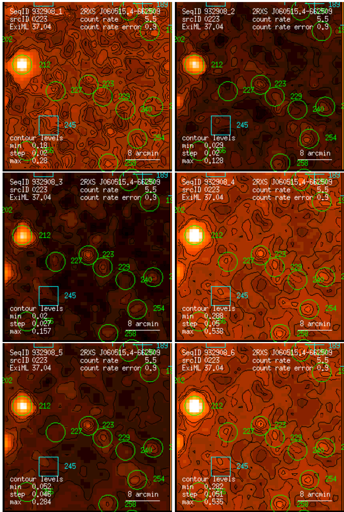
Figure 223: RASS 932908: detection 0223: band rate images, Gaussian filter: (1) PSPC channels 11 – 41, (2) 52 – 90, (3) 91 – 201, (4) 11 – 235, (5) 52 – 201, (6) 11 – 201. Broad band rates in counts/ks. Band rate contour levels in counts/ks/arcmin 2 .
