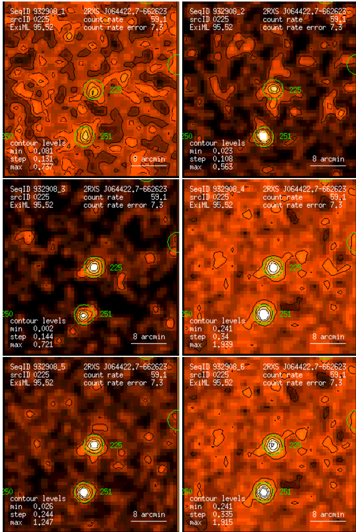
Figure 225: RASS 932908: detection 0225: band rate images, Gaussian filter: (1) PSPC channels 11 – 41, (2) 52 – 90, (3) 91 – 201, (4) 11 – 235, (5) 52 – 201, (6) 11 – 201. Broad band rates in counts/ks. Band rate contour levels in counts/ks/arcmin 2 .
