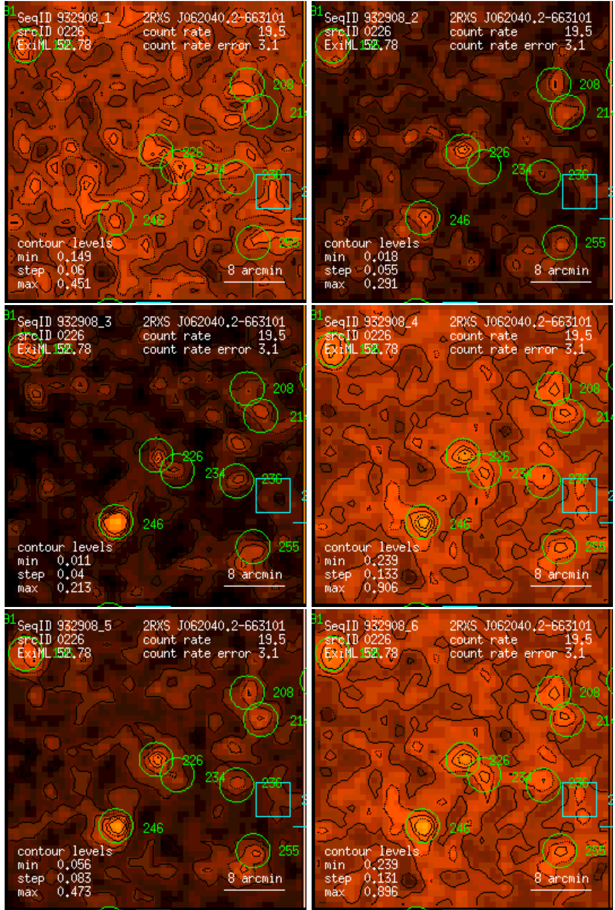
Figure 226: RASS 932908: detection 0226: band rate images, Gaussian filter: (1) PSPC channels 11 – 41, (2) 52 – 90, (3) 91 – 201, (4) 11 – 235, (5) 52 – 201, (6) 11 – 201. Broad band rates in counts/ks. Band rate contour levels in counts/ks/arcmin 2 .
