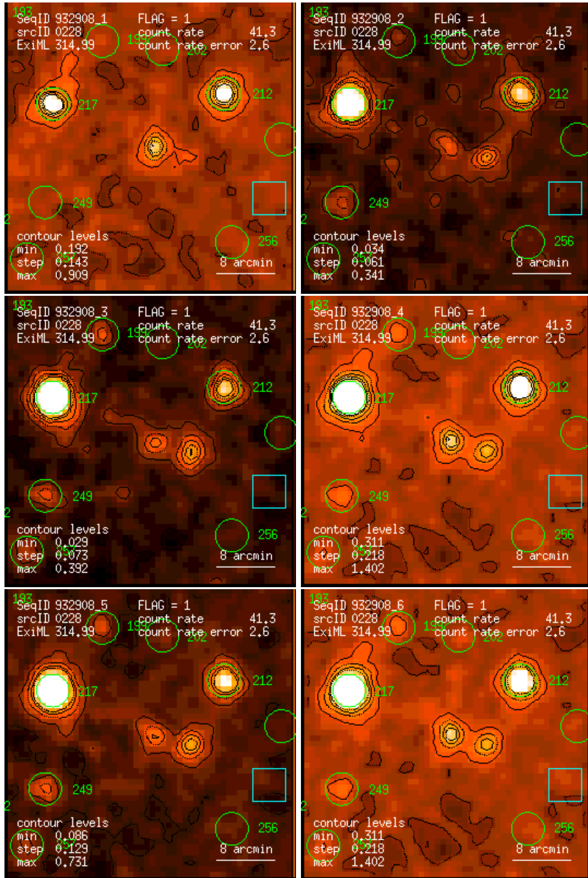
Figure 228: RASS 932908: detection 0228: band rate images, Gaussian filter: (1) PSPC channels 11 – 41, (2) 52 – 90, (3) 91 – 201, (4) 11 – 235, (5) 52 – 201, (6) 11 – 201. Broad band rates in counts/ks. Band rate contour levels in counts/ks/arcmin 2 .
