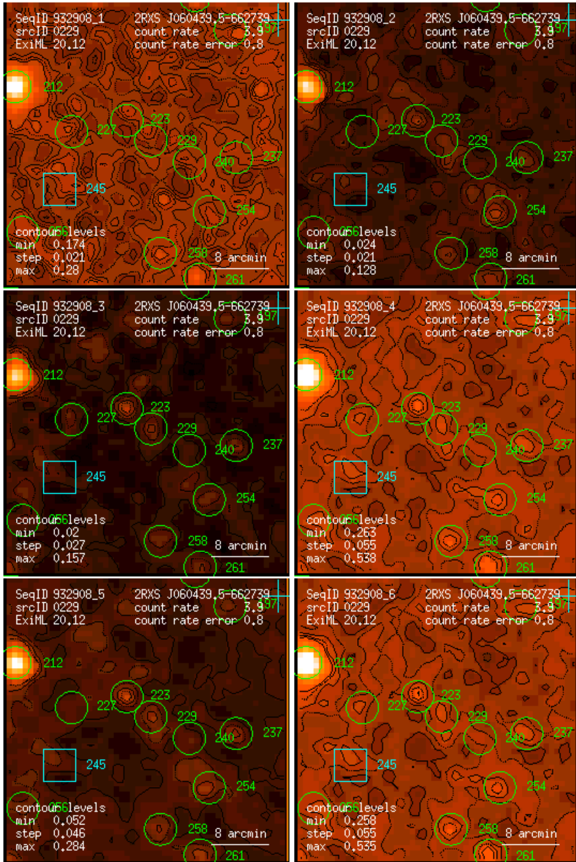
Figure 229: RASS 932908: detection 0229: band rate images, Gaussian filter: (1) PSPC channels 11 – 41, (2) 52 – 90, (3) 91 – 201, (4) 11 – 235, (5) 52 – 201, (6) 11 – 201. Broad band rates in counts/ks. Band rate contour levels in counts/ks/arcmin 2 .
