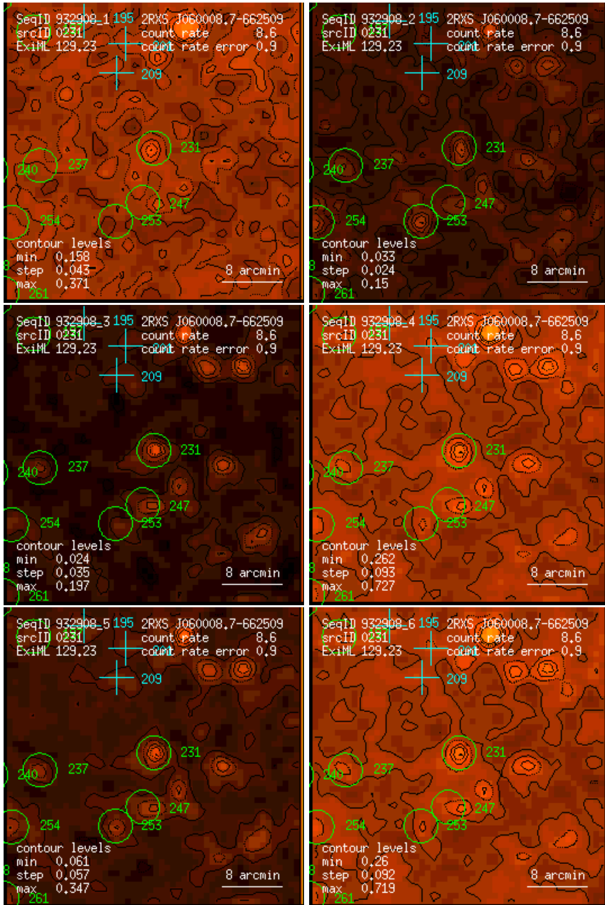
Figure 231: RASS 932908: detection 0231: band rate images, Gaussian filter: (1) PSPC channels 11 – 41, (2) 52 – 90, (3) 91 – 201, (4) 11 – 235, (5) 52 – 201, (6) 11 – 201. Broad band rates in counts/ks. Band rate contour levels in counts/ks/arcmin 2 .
