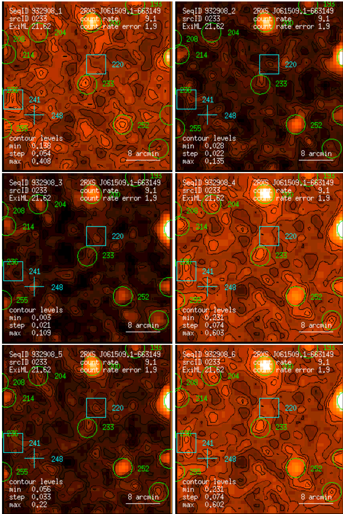
Figure 233: RASS 932908: detection 0233: band rate images, Gaussian filter: (1) PSPC channels 11 – 41, (2) 52 – 90, (3) 91 – 201, (4) 11 – 235, (5) 52 – 201, (6) 11 – 201. Broad band rates in counts/ks. Band rate contour levels in counts/ks/arcmin 2 .
