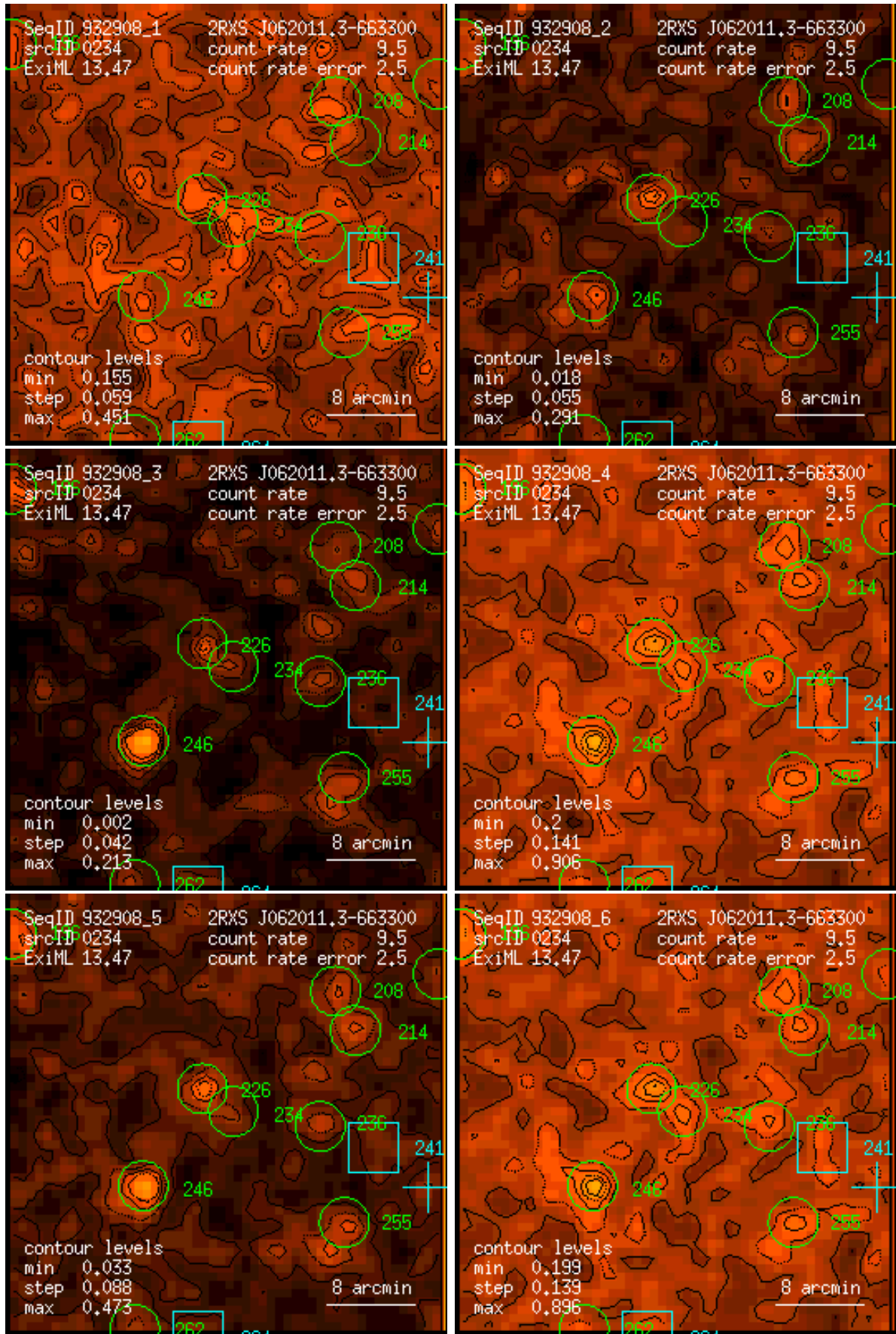
Figure 234: RASS 932908: detection 0234: band rate images, Gaussian filter: (1) PSPC channels 11 – 41, (2) 52 – 90, (3) 91 – 201, (4) 11 – 235, (5) 52 – 201, (6) 11 – 201. Broad band rates in counts/ks. Band rate contour levels in counts/ks/arcmin 2 .
