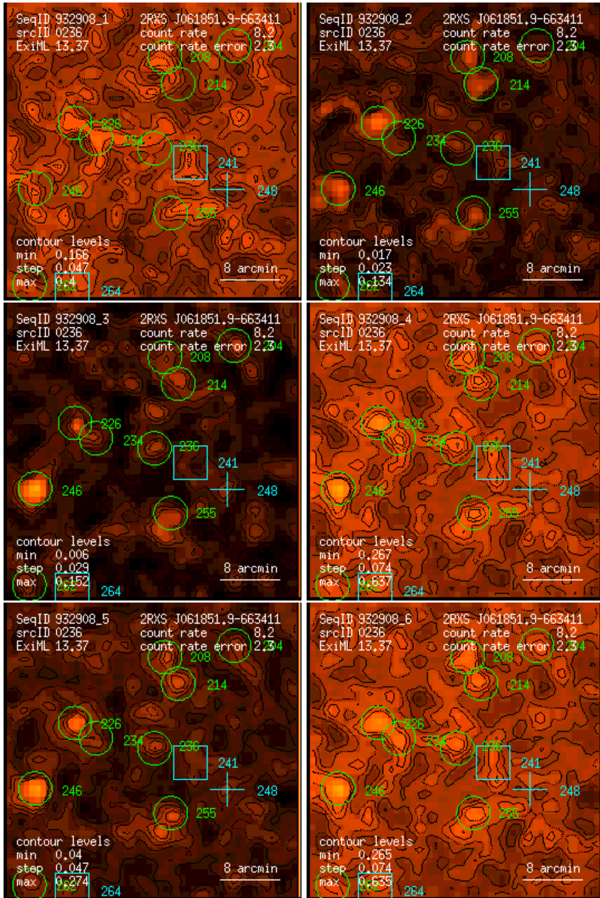
Figure 236: RASS 932908: detection 0236: band rate images, Gaussian filter: (1) PSPC channels 11 – 41, (2) 52 – 90, (3) 91 – 201, (4) 11 – 235, (5) 52 – 201, (6) 11 – 201. Broad band rates in counts/ks. Band rate contour levels in counts/ks/arcmin 2 .
