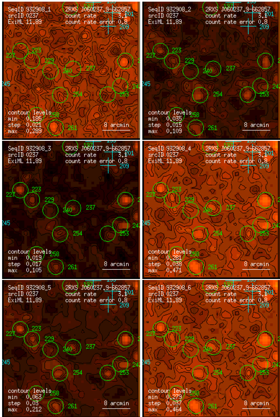
Figure 237: RASS 932908: detection 0237: band rate images, Gaussian filter: (1) PSPC channels 11 – 41, (2) 52 – 90, (3) 91 – 201, (4) 11 – 235, (5) 52 – 201, (6) 11 – 201. Broad band rates in counts/ks. Band rate contour levels in counts/ks/arcmin 2 .
