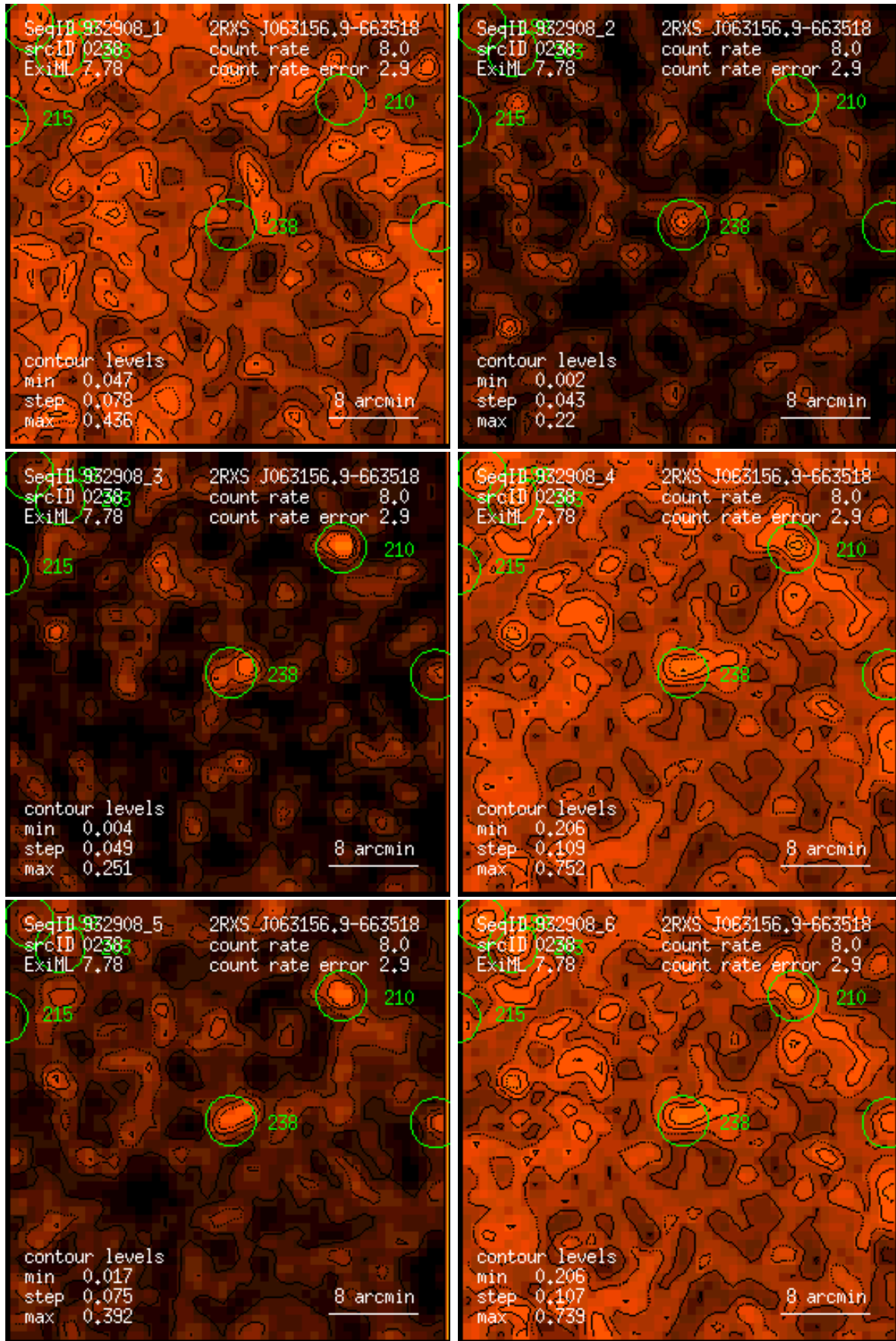
Figure 238: RASS 932908: detection 0238: band rate images, Gaussian filter: (1) PSPC channels 11 – 41, (2) 52 – 90, (3) 91 – 201, (4) 11 – 235, (5) 52 – 201, (6) 11 – 201. Broad band rates in counts/ks. Band rate contour levels in counts/ks/arcmin 2 .
