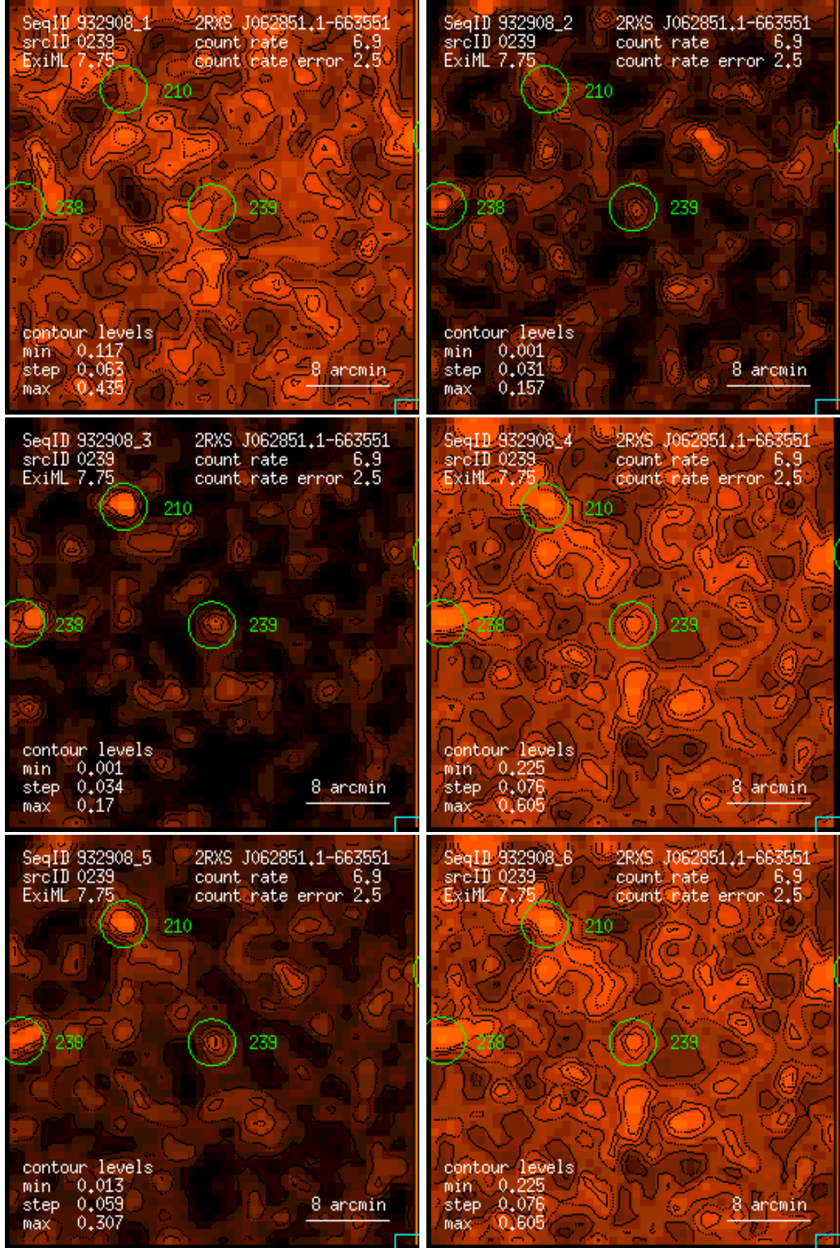
Figure 239: RASS 932908: detection 0239: band rate images, Gaussian filter: (1) PSPC channels 11 – 41, (2) 52 – 90, (3) 91 – 201, (4) 11 – 235, (5) 52 – 201, (6) 11 – 201. Broad band rates in counts/ks. Band rate contour levels in counts/ks/arcmin 2 .
