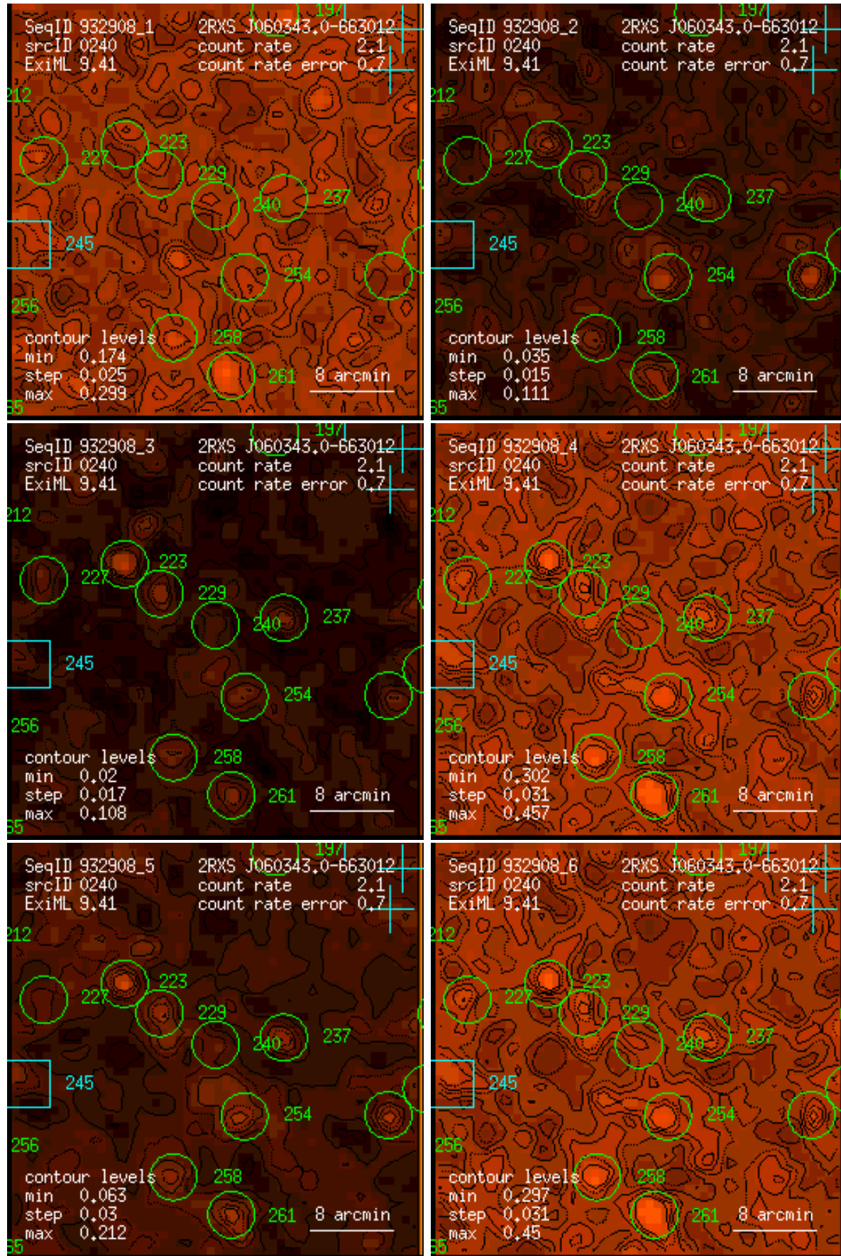
Figure 240: RASS 932908: detection 0240: band rate images, Gaussian filter: (1) PSPC channels 11 – 41, (2) 52 – 90, (3) 91 – 201, (4) 11 – 235, (5) 52 – 201, (6) 11 – 201. Broad band rates in counts/ks. Band rate contour levels in counts/ks/arcmin 2 .
