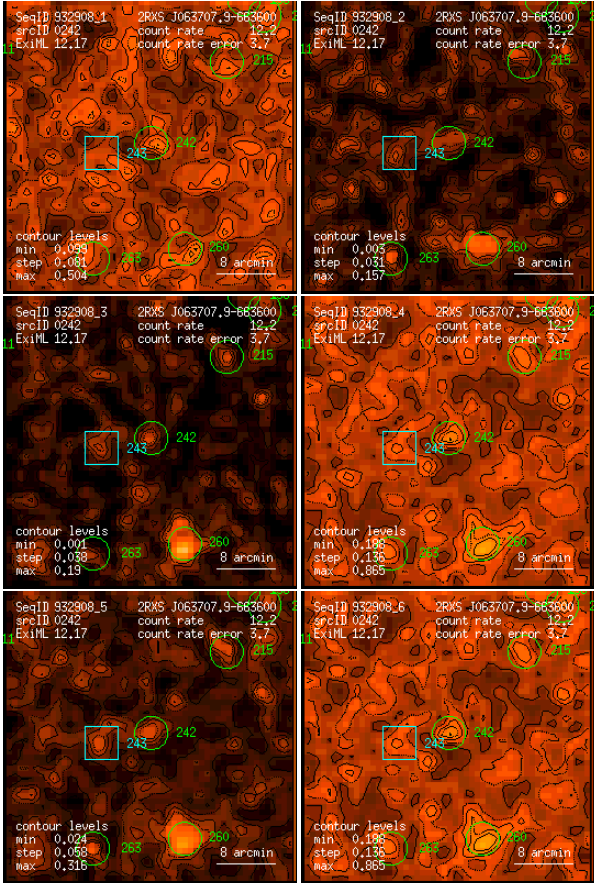
Figure 242: RASS 932908: detection 0242: band rate images, Gaussian filter: (1) PSPC channels 11 – 41, (2) 52 – 90, (3) 91 – 201, (4) 11 – 235, (5) 52 – 201, (6) 11 – 201. Broad band rates in counts/ks. Band rate contour levels in counts/ks/arcmin 2 .
