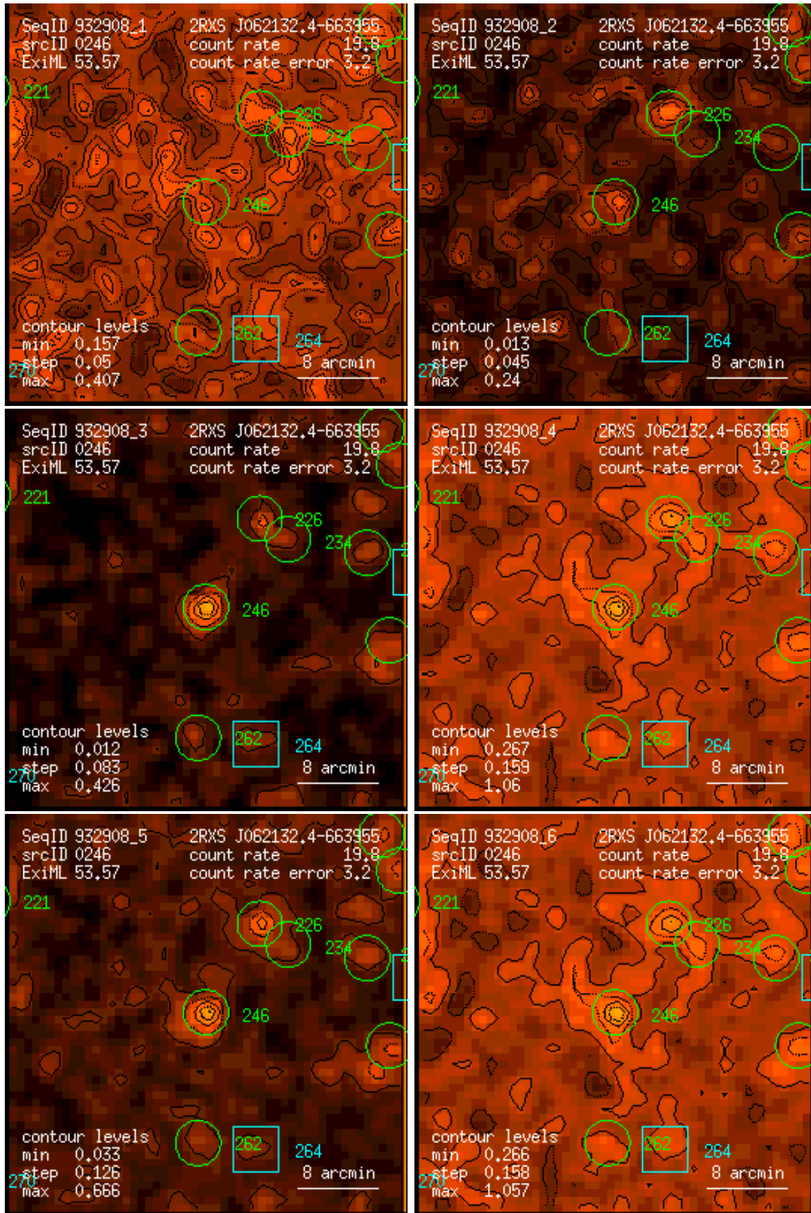
Figure 246: RASS 932908: detection 0246: band rate images, Gaussian filter: (1) PSPC channels 11 – 41, (2) 52 – 90, (3) 91 – 201, (4) 11 – 235, (5) 52 – 201, (6) 11 – 201. Broad band rates in counts/ks. Band rate contour levels in counts/ks/arcmin 2 .
