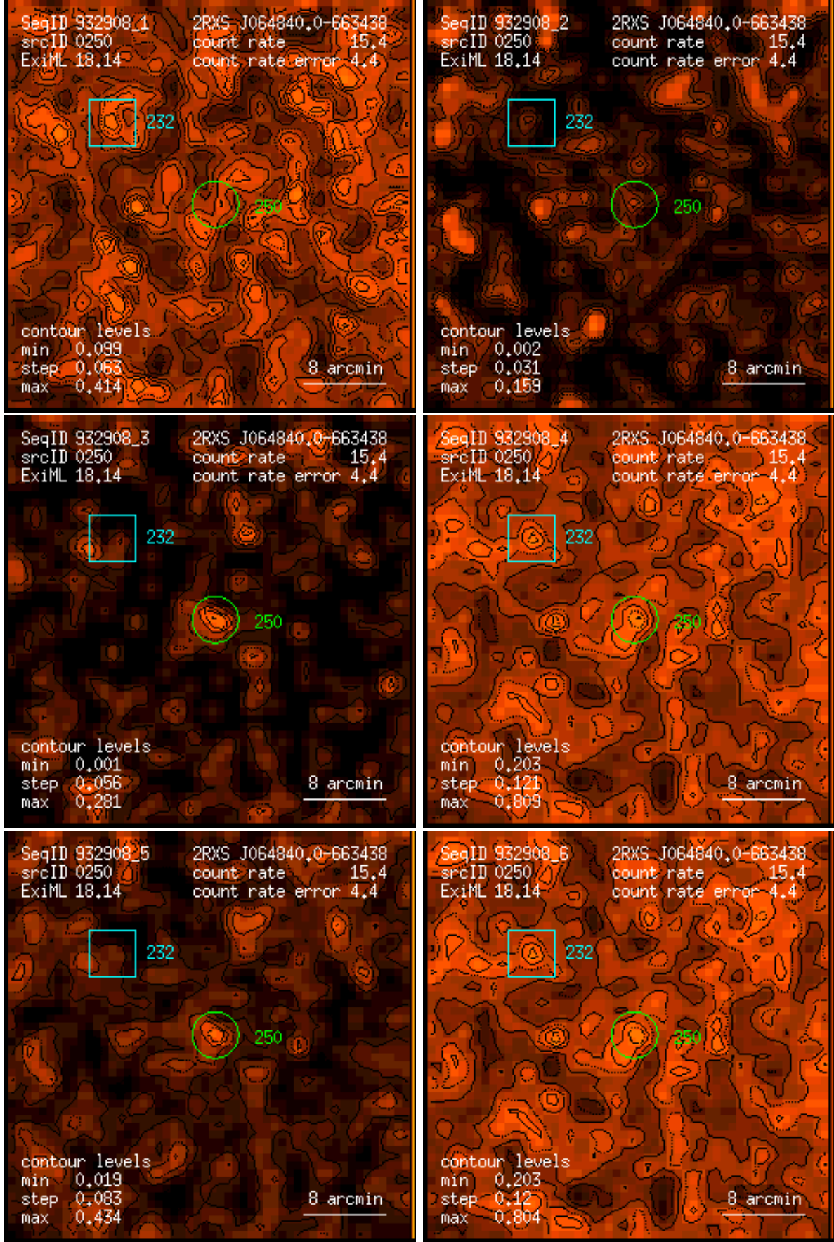
Figure 250: RASS 932908: detection 0250: band rate images, Gaussian filter: (1) PSPC channels 11 – 41, (2) 52 – 90, (3) 91 – 201, (4) 11 – 235, (5) 52 – 201, (6) 11 – 201. Broad band rates in counts/ks. Band rate contour levels in counts/ks/arcmin 2 .
