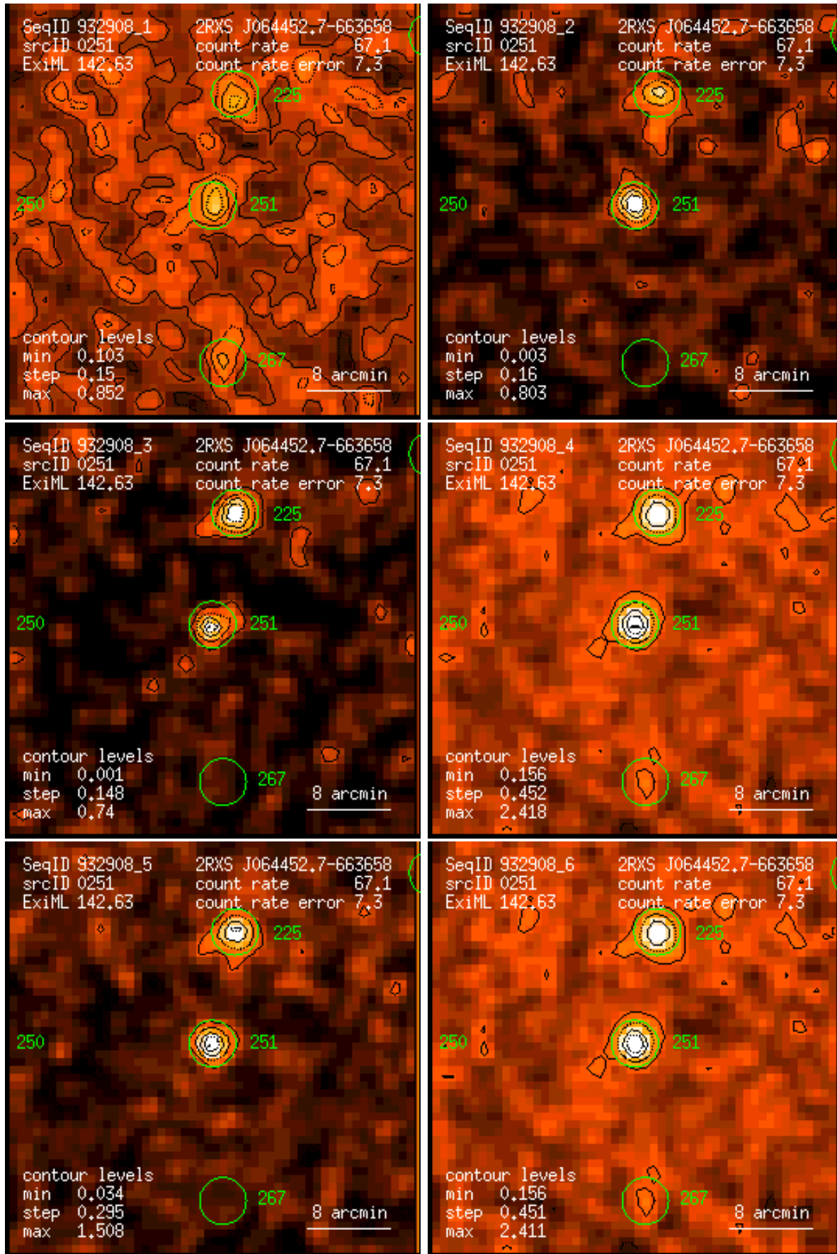
Figure 251: RASS 932908: detection 0251: band rate images, Gaussian filter: (1) PSPC channels 11 – 41, (2) 52 – 90, (3) 91 – 201, (4) 11 – 235, (5) 52 – 201, (6) 11 – 201. Broad band rates in counts/ks. Band rate contour levels in counts/ks/arcmin 2 .
