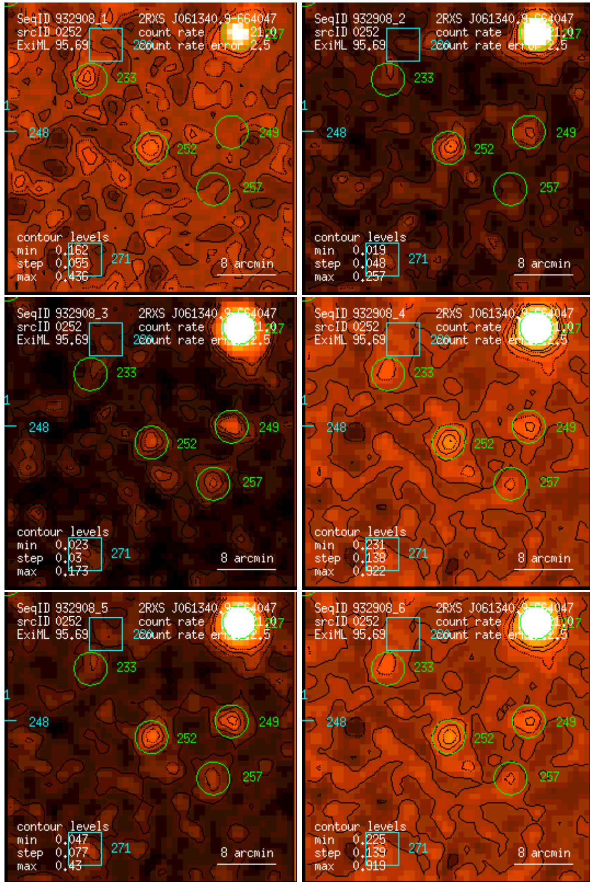
Figure 252: RASS 932908: detection 0252: band rate images, Gaussian filter: (1) PSPC channels 11 – 41, (2) 52 – 90, (3) 91 – 201, (4) 11 – 235, (5) 52 – 201, (6) 11 – 201. Broad band rates in counts/ks. Band rate contour levels in counts/ks/arcmin 2 .
