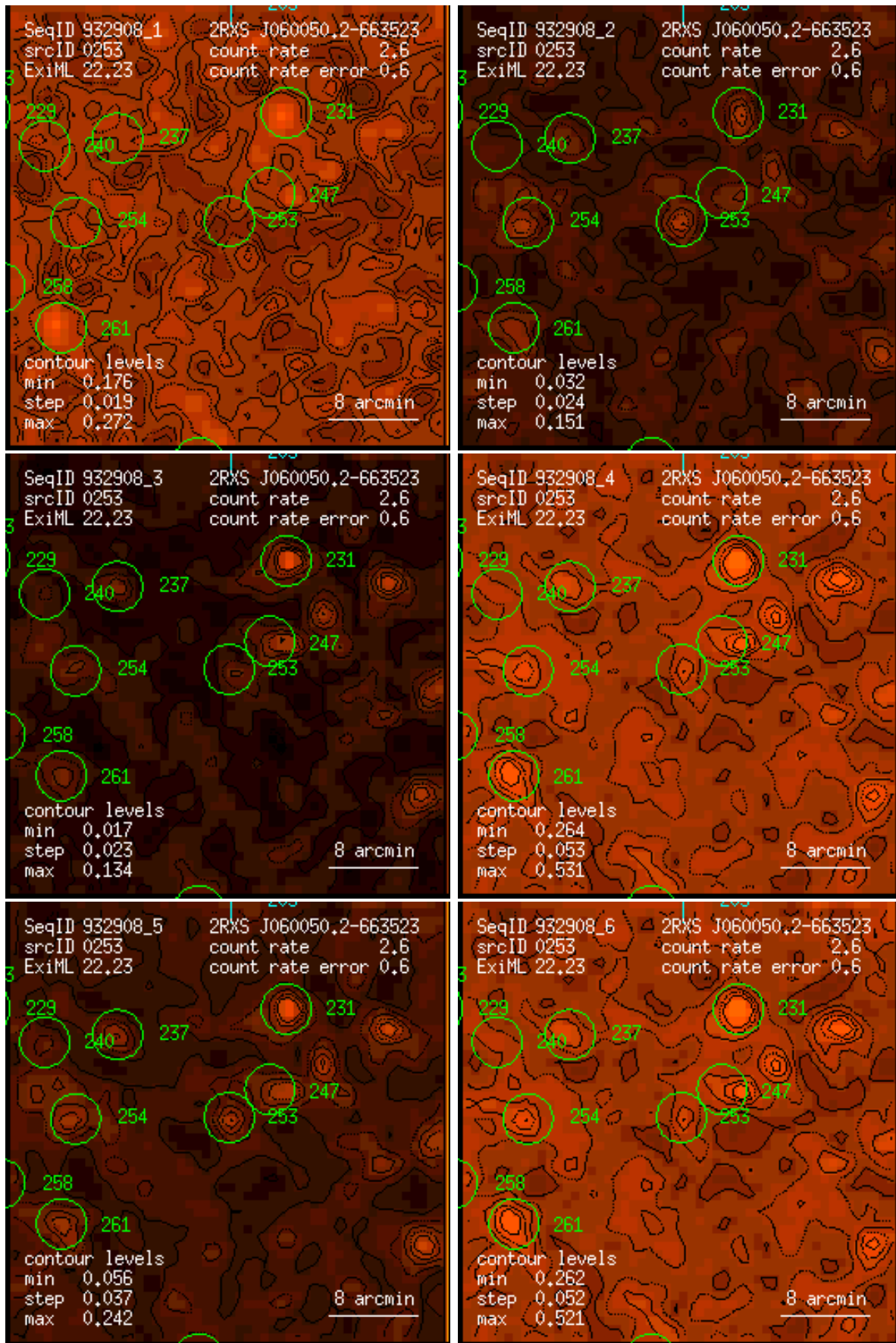
Figure 253: RASS 932908: detection 0253: band rate images, Gaussian filter: (1) PSPC channels 11 – 41, (2) 52 – 90, (3) 91 – 201, (4) 11 – 235, (5) 52 – 201, (6) 11 – 201. Broad band rates in counts/ks. Band rate contour levels in counts/ks/arcmin 2 .
