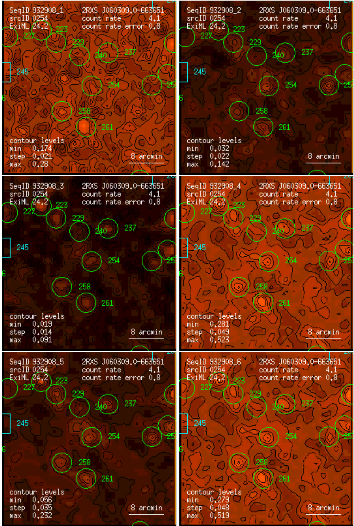
Figure 254: RASS 932908: detection 0254: band rate images, Gaussian filter: (1) PSPC channels 11 – 41, (2) 52 – 90, (3) 91 – 201, (4) 11 – 235, (5) 52 – 201, (6) 11 – 201. Broad band rates in counts/ks. Band rate contour levels in counts/ks/arcmin 2 .
