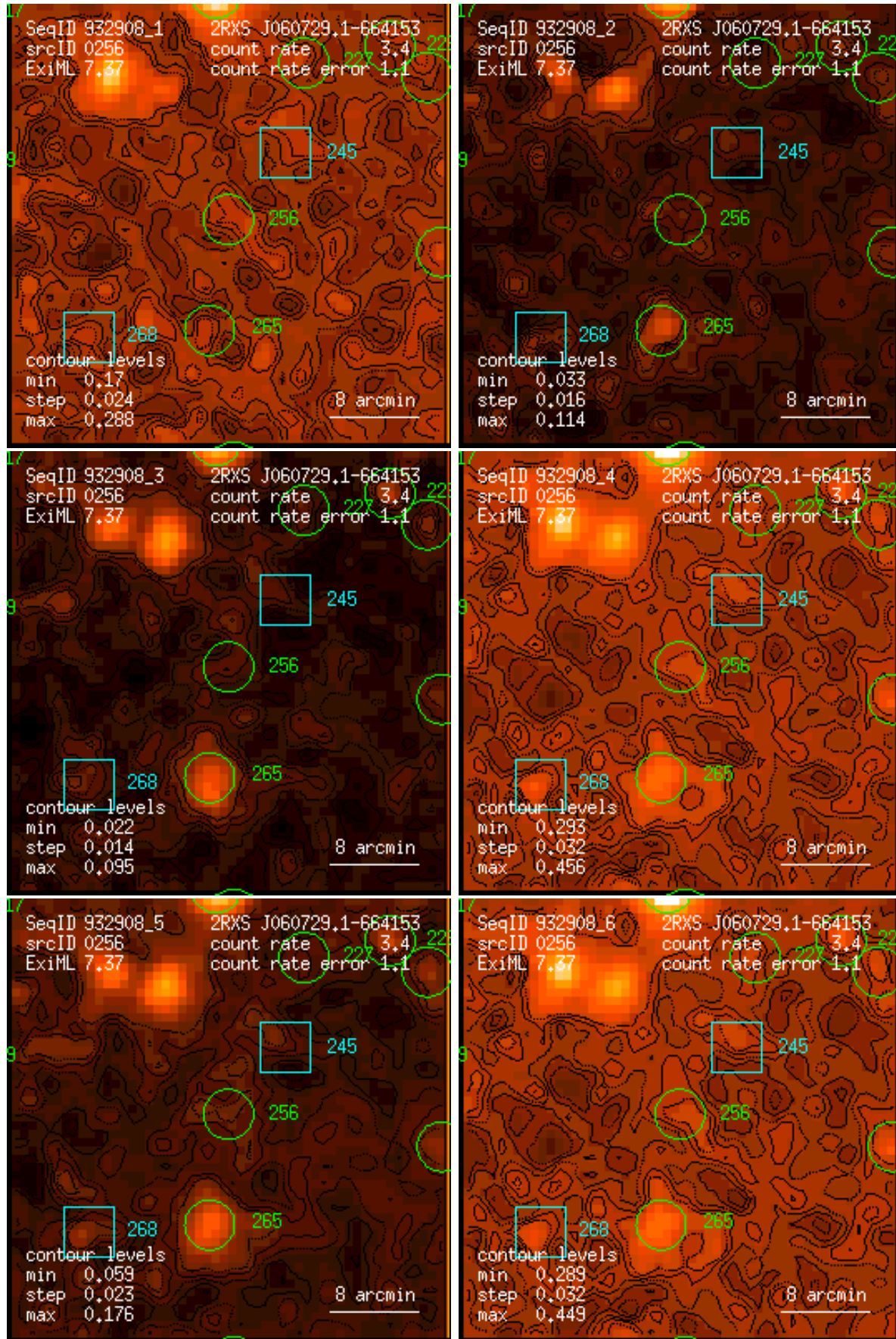
Figure 256: RASS 932908: detection 0256: band rate images, Gaussian filter: (1) PSPC channels 11 – 41, (2) 52 – 90, (3) 91 – 201, (4) 11 – 235, (5) 52 – 201, (6) 11 – 201. Broad band rates in counts/ks. Band rate contour levels in counts/ks/arcmin 2 .
