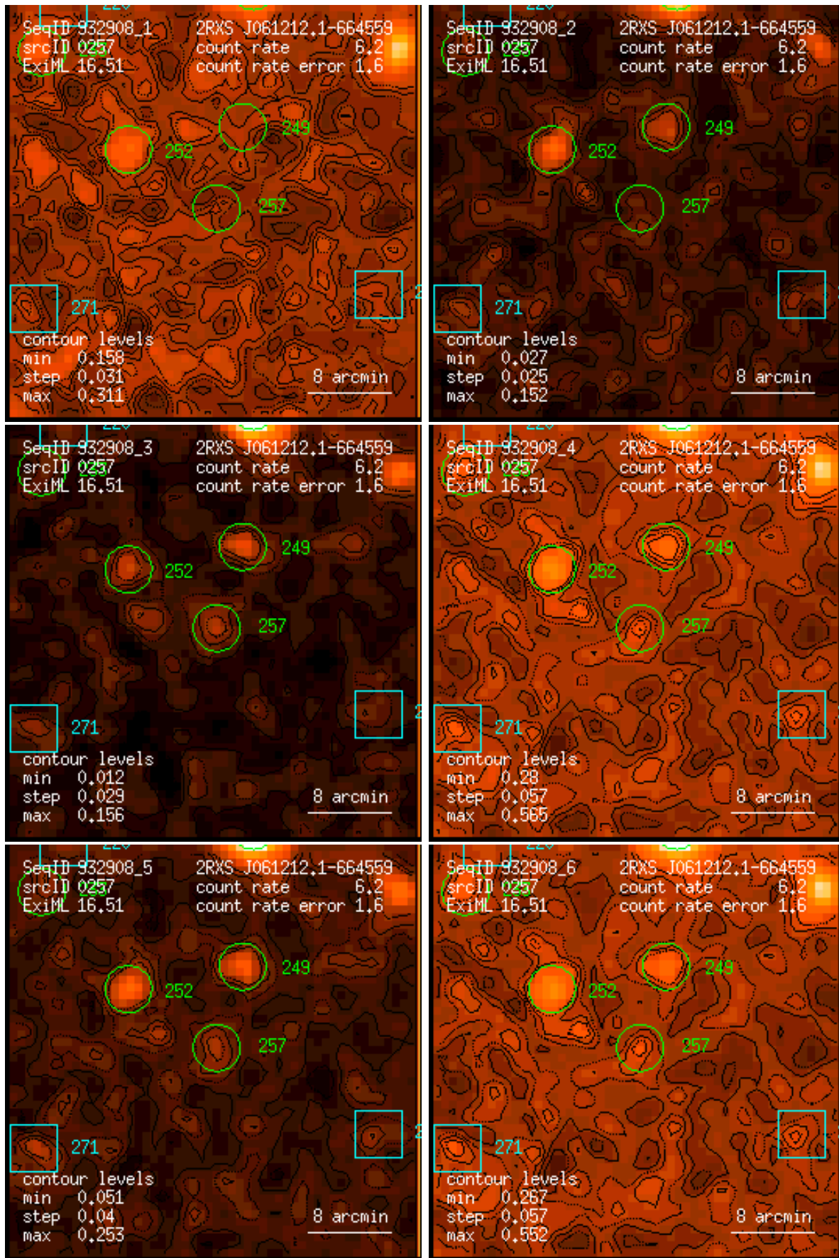
Figure 257: RASS 932908: detection 0257: band rate images, Gaussian filter: (1) PSPC channels 11 – 41, (2) 52 – 90, (3) 91 – 201, (4) 11 – 235, (5) 52 – 201, (6) 11 – 201. Broad band rates in counts/ks. Band rate contour levels in counts/ks/arcmin 2 .
