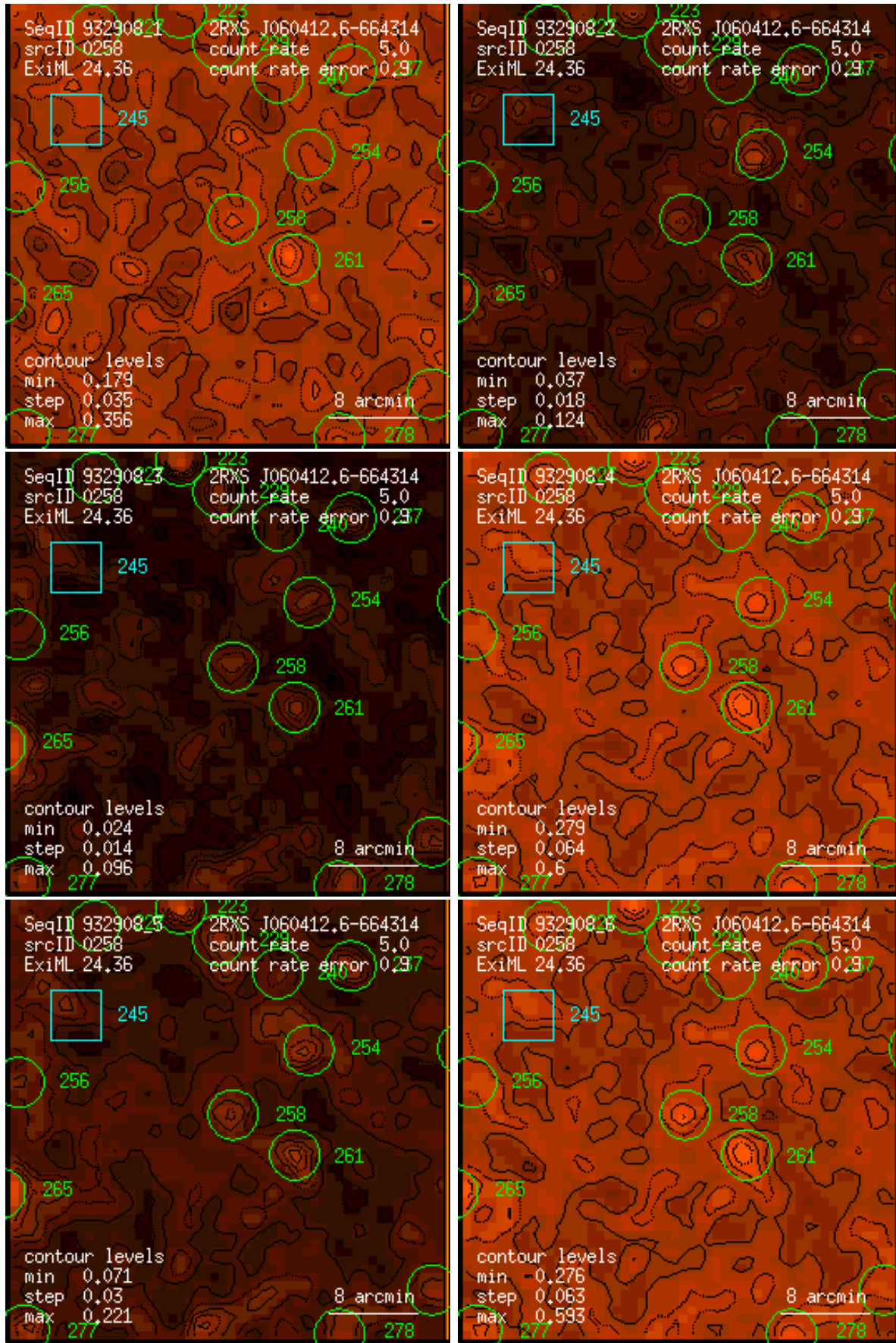
Figure 258: RASS 932908: detection 0258: band rate images, Gaussian filter: (1) PSPPC channels 11 – 41, (2) 52 – 90, (3) 91 – 201, (4) 11 – 235, (5) 52 – 201, (6) 11 – 201. Broad band rates in counts/ks. Band rate contour levels in counts/ks/arcmin 2 .
