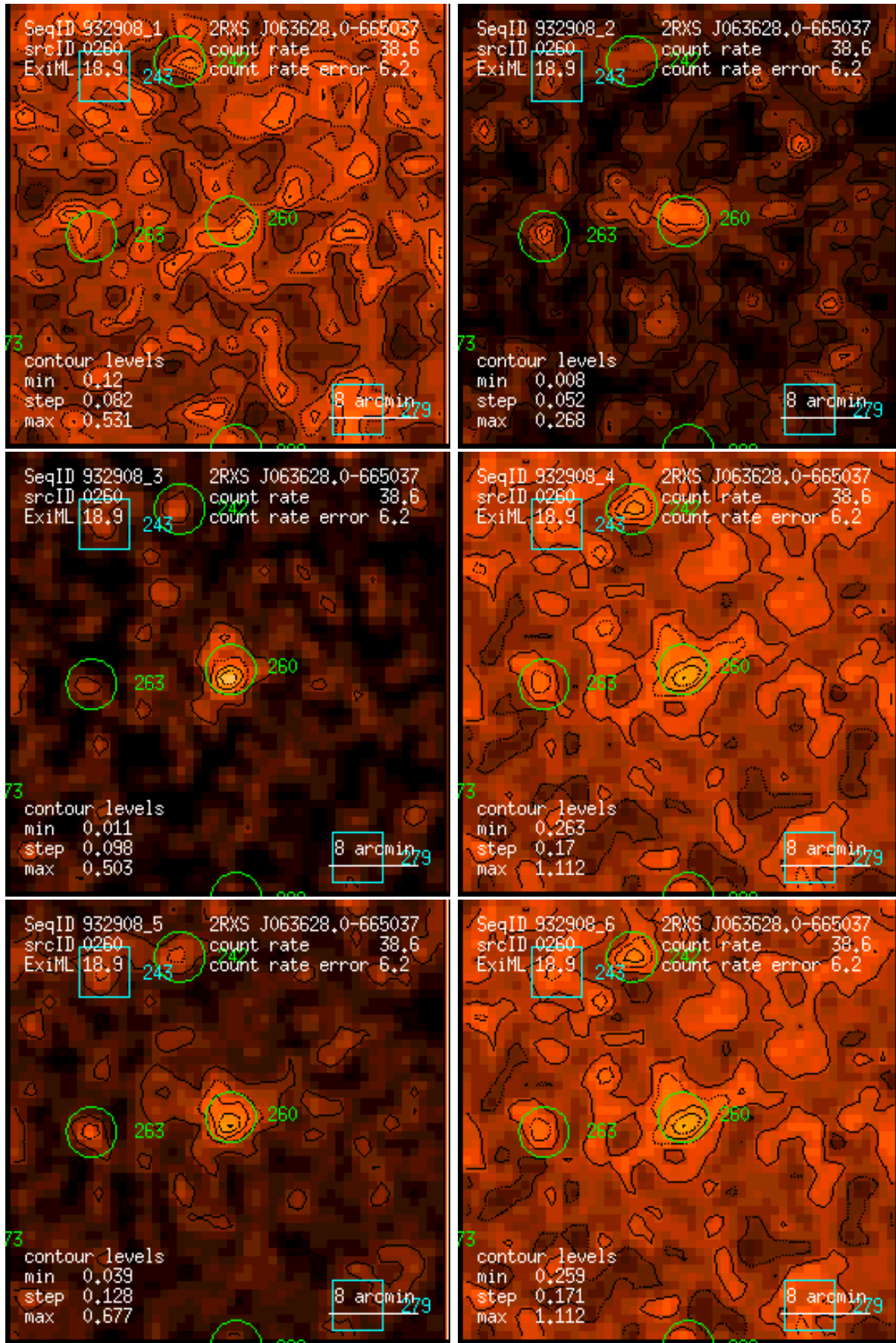
Figure 260: RASS 932908: detection 0260: band rate images, Gaussian filter: (1) PSPC channels 11 – 41, (2) 52 – 90, (3) 91 – 201, (4) 11 – 235, (5) 52 – 201, (6) 11 – 201. Broad band rates in counts/ks. Band rate contour levels in counts/ks/arcmin 2 .
