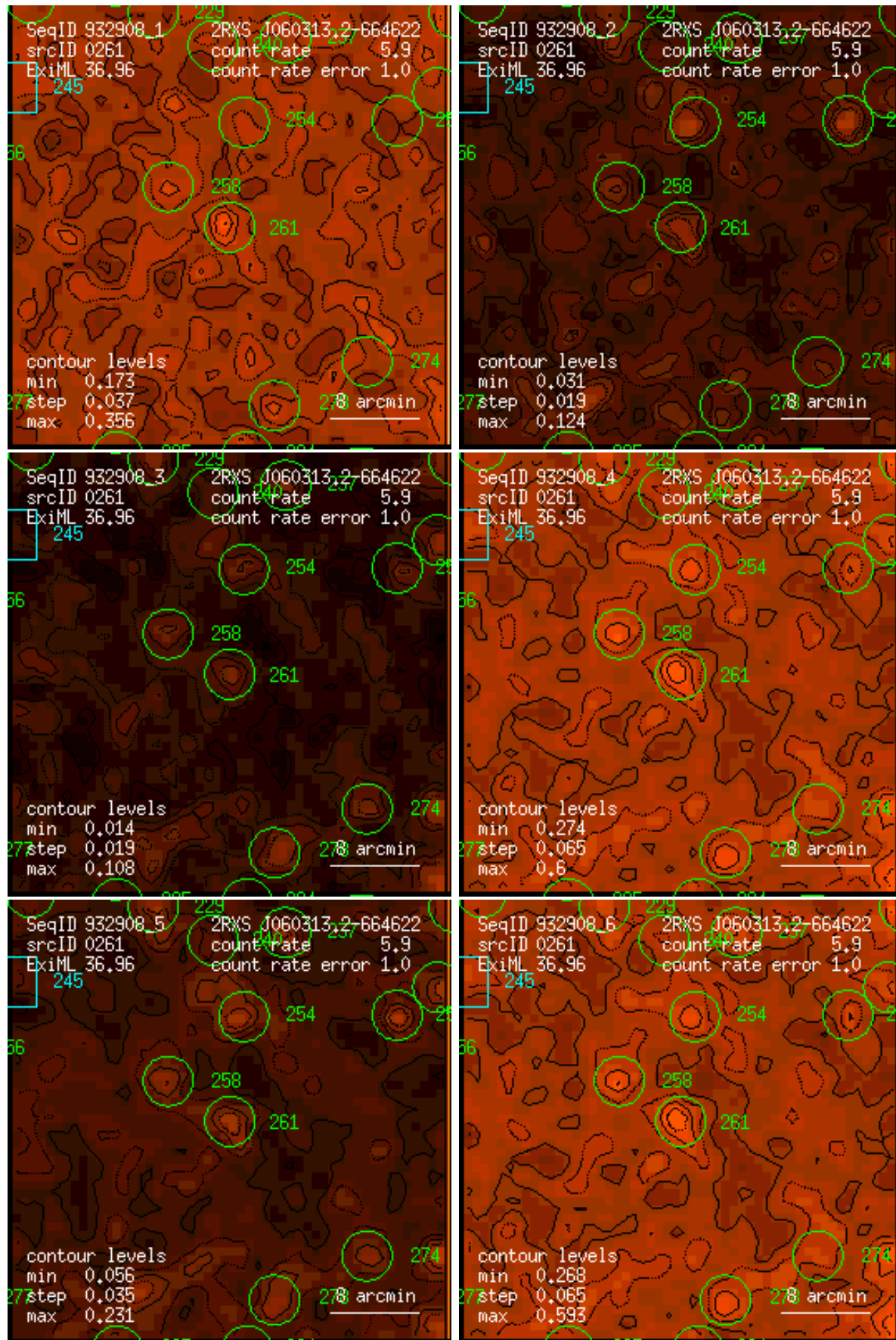
Figure 261: RASS 932908: detection 0261: band rate images, Gaussian filter: (1) PSPC channels 11 – 41, (2) 52 – 90, (3) 91 – 201, (4) 11 – 235, (5) 52 – 201, (6) 11 – 201. Broad band rates in counts/ks. Band rate contour levels in counts/ks/arcmin 2 .
