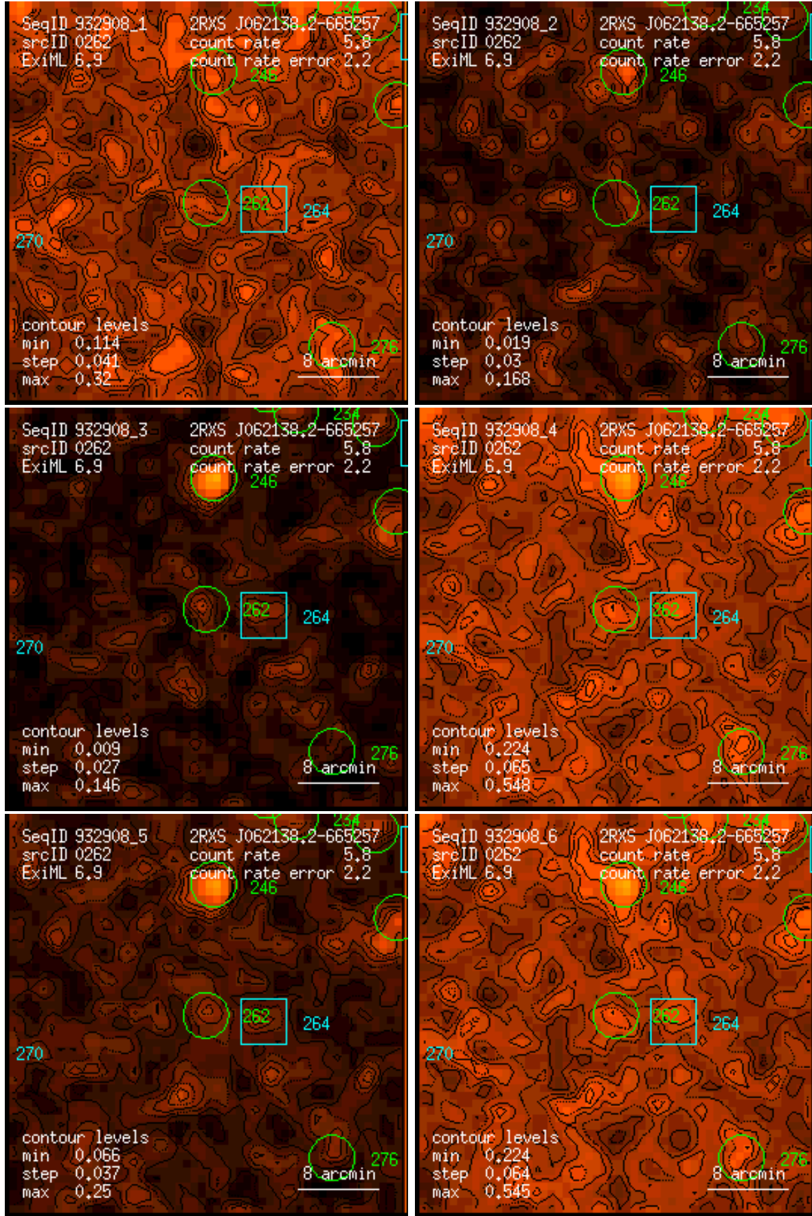
Figure 262: RASS 932908: detection 0262: band rate images, Gaussian filter: (1) PSPC channels 11 – 41, (2) 52 – 90, (3) 91 – 201, (4) 11 – 235, (5) 52 – 201, (6) 11 – 201. Broad band rates in counts/ks. Band rate contour levels in counts/ks/arcmin 2 .
