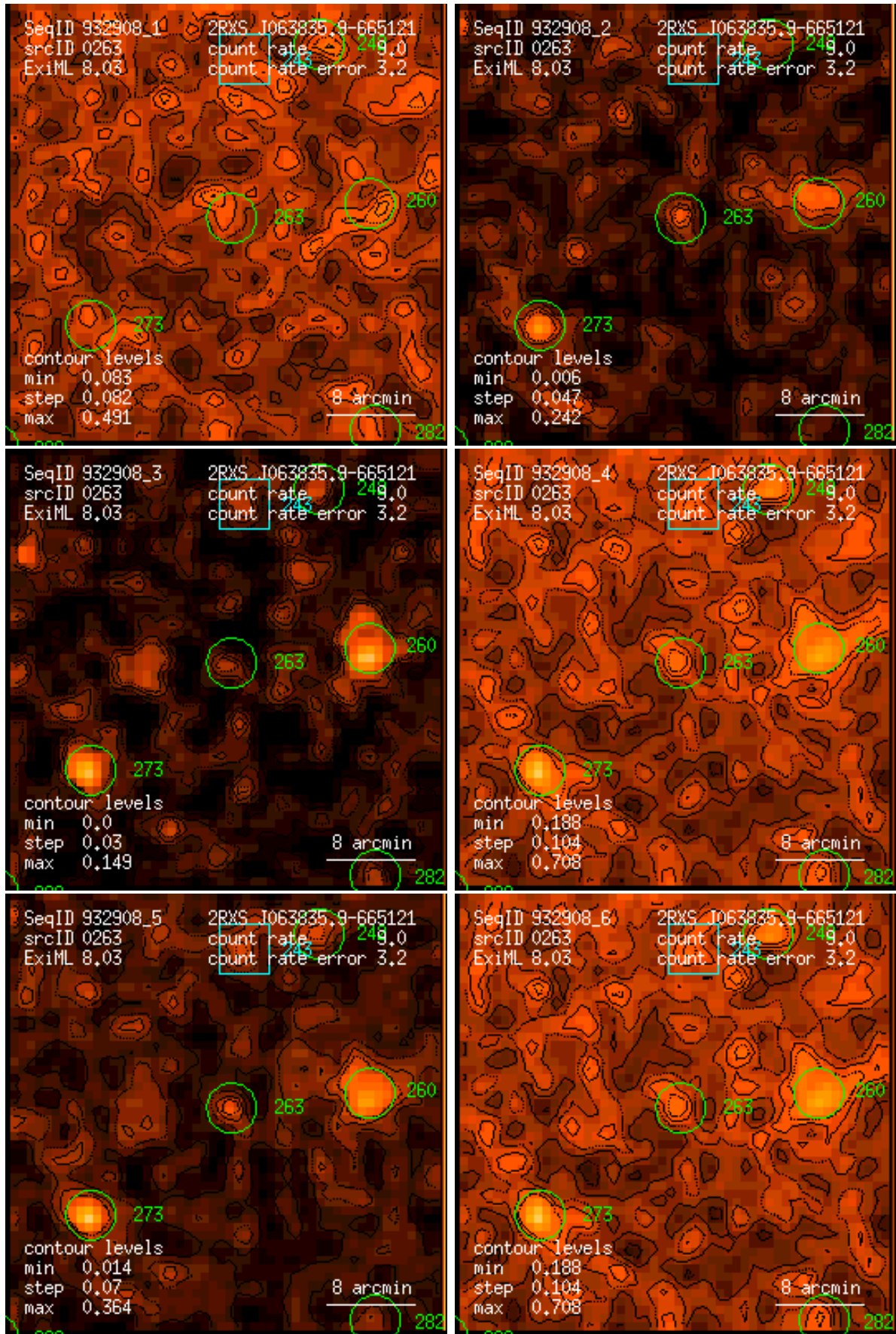
Figure 263: RASS 932908: detection 0263: band rate images, Gaussian filter: (1) PSPC channels 11 – 41, (2) 52 – 90, (3) 91 – 201, (4) 11 – 235, (5) 52 – 201, (6) 11 – 201. Broad band rates in counts/ks. Band rate contour levels in counts/ks/arcmin 2 .
