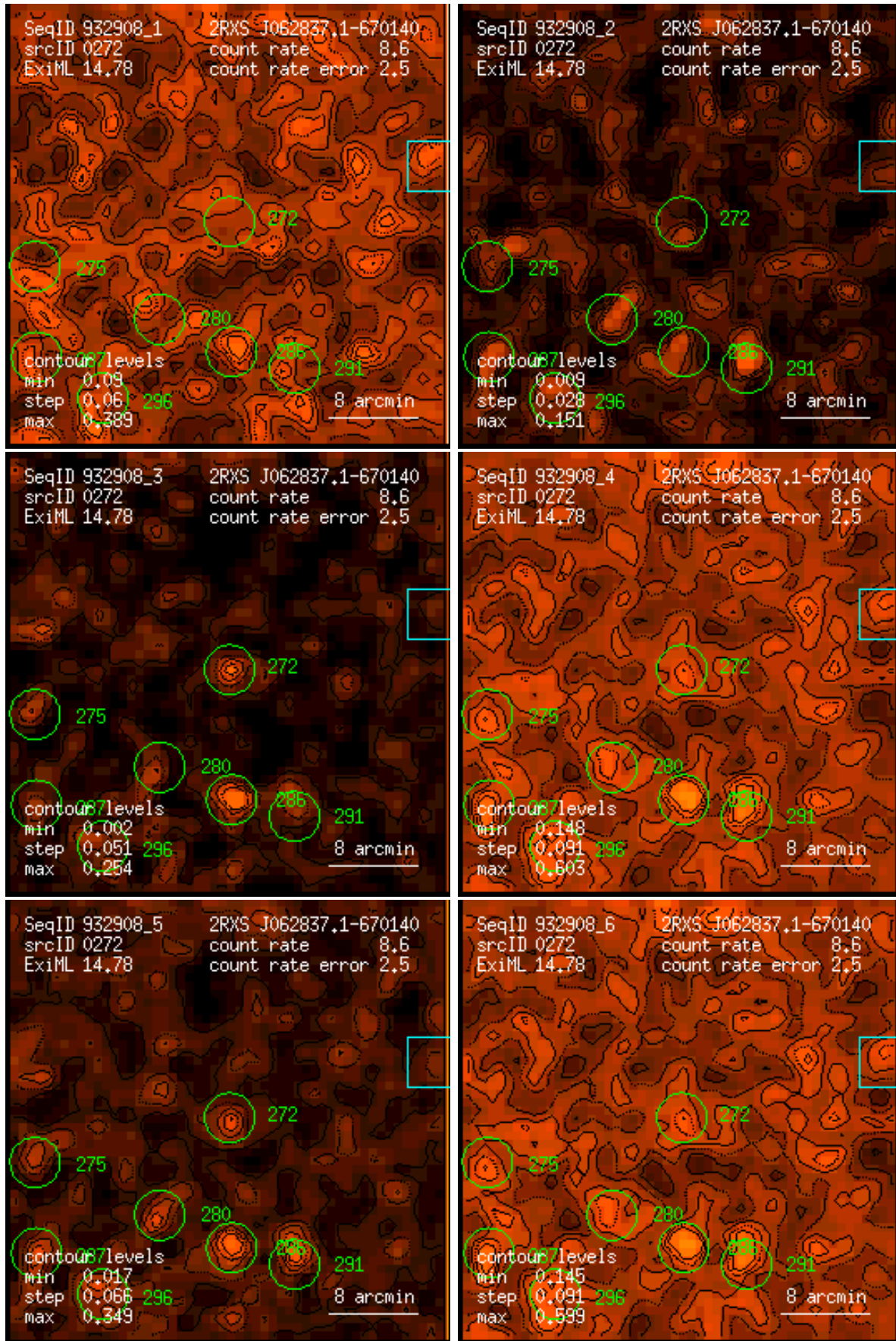
Figure 272: RASS 932908: detection 0272: band rate images, Gaussian filter: (1) PSPPC channels 11 – 41, (2) 52 – 90, (3) 91 – 201, (4) 11 – 235, (5) 52 – 201, (6) 11 – 201. Broad band rates in counts/ks. Band rate contour levels in counts/ks/arcmin 2 .
